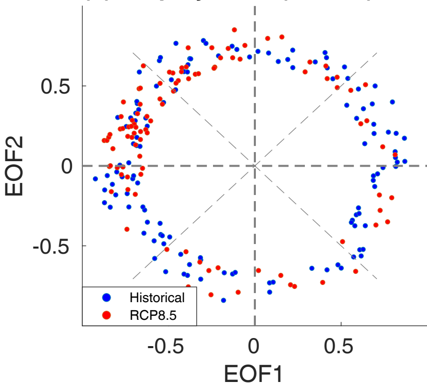
(b) AS projection (MIROC)
