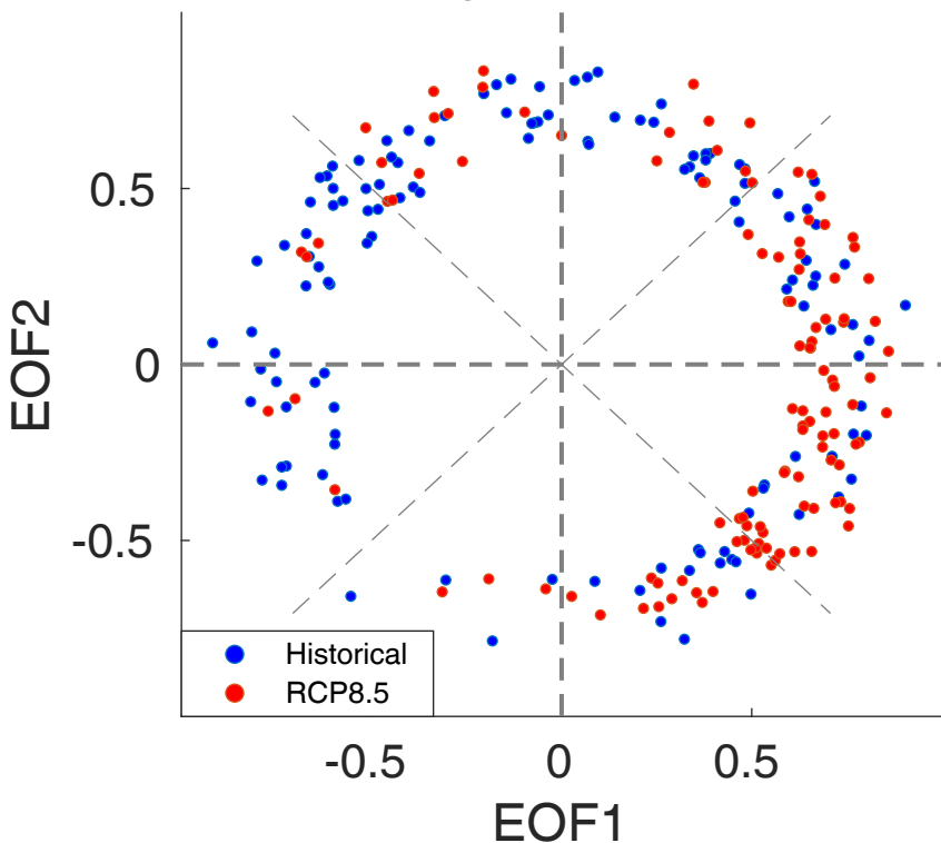
(a) NA projection (IPSL)
