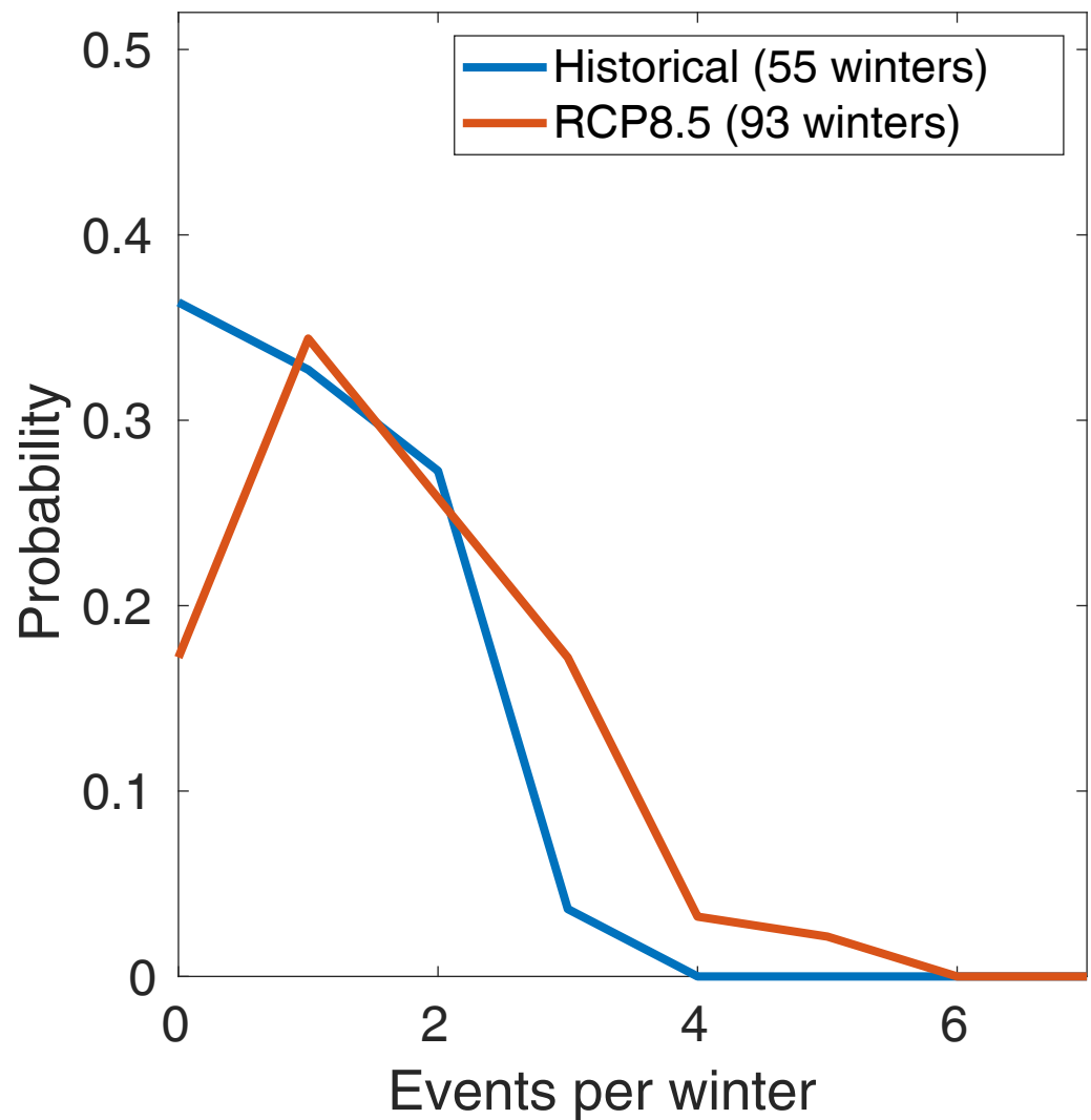
(b) AS CTP events PDF (MIROC)
