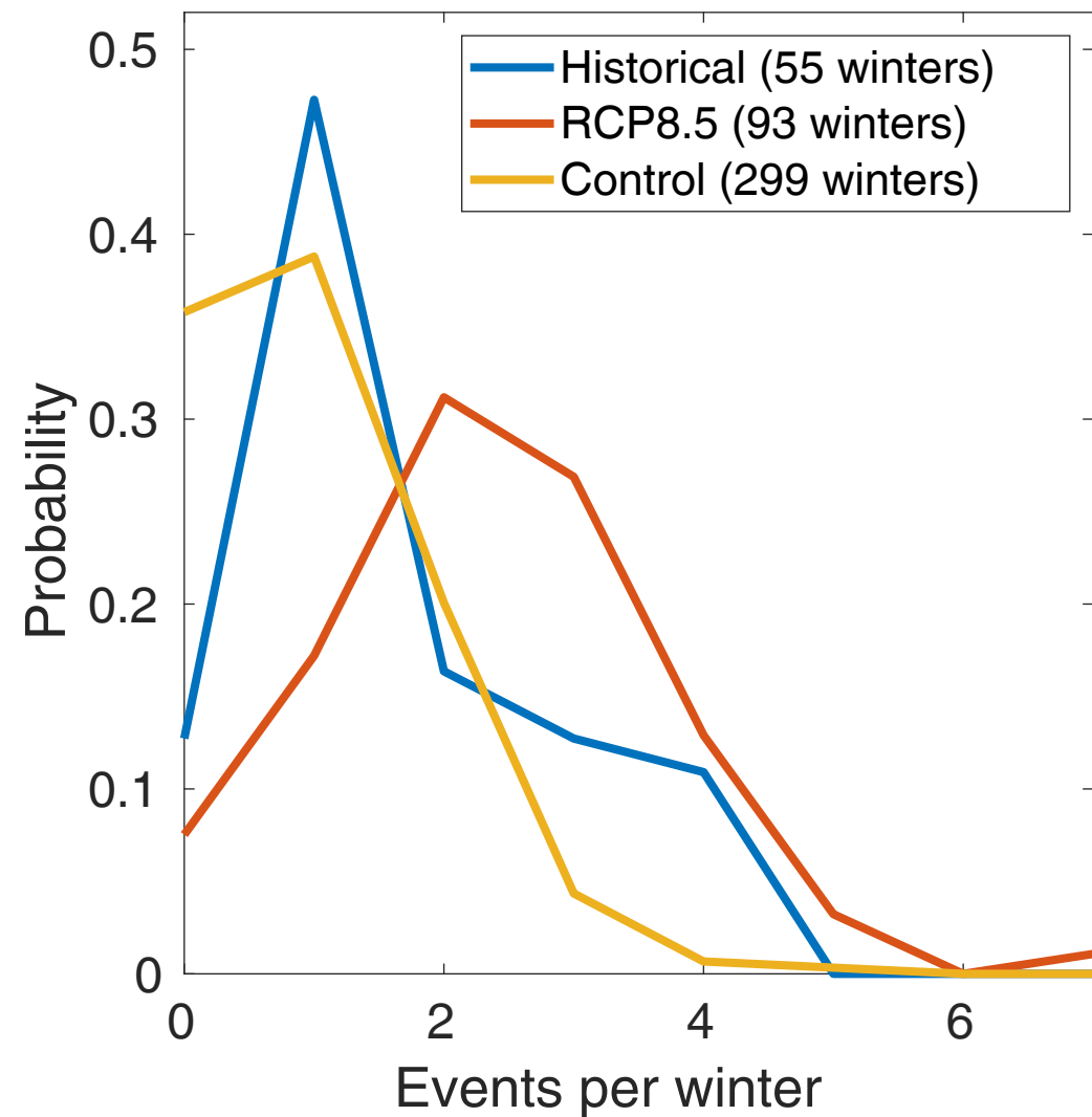
(a) NA CTP events PDF (IPSL)
