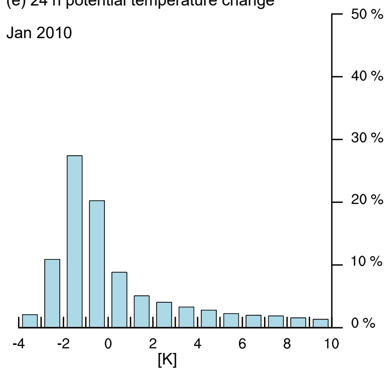
(e) 24 h potential temperature change
