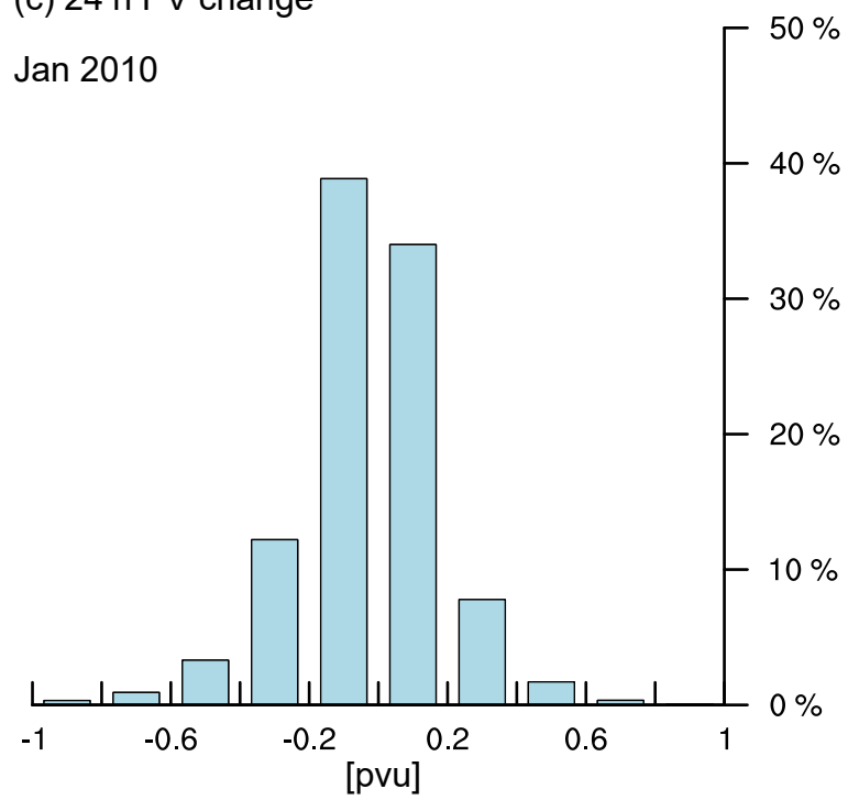
(c) 24 h PV change
