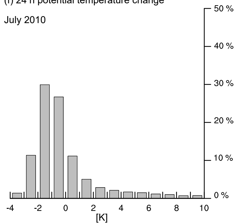
(f) 24 h potential temperature change
