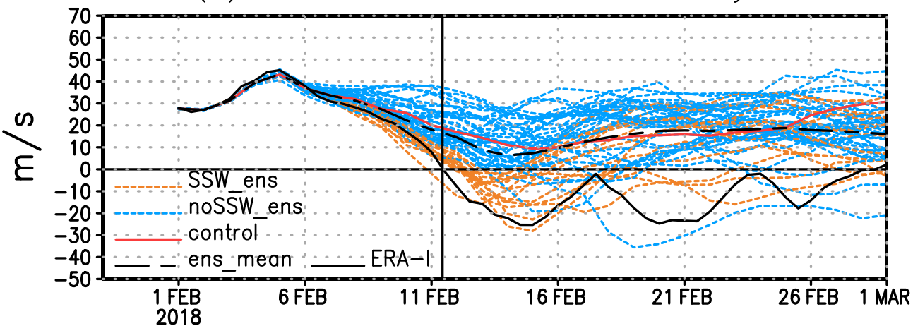
(b) U10, forecast from 1 February
