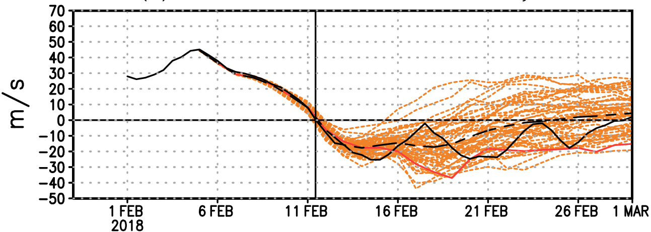
(c) U10, forecast from 5 February
