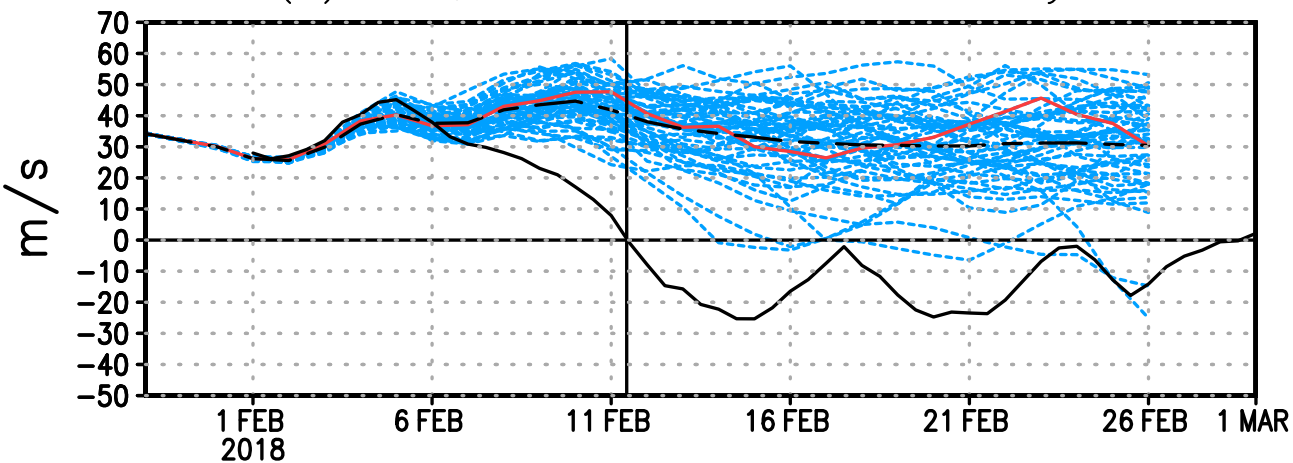
(a) U10, forecast from 29 January
