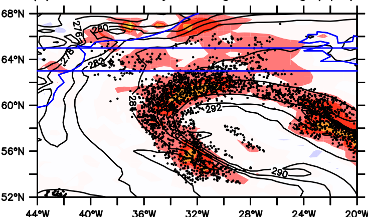
(e) NoConv, vertically-averaged heating (K/h)
