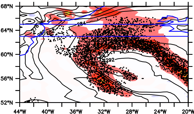
(c) PCMT, vertically-averaged heating (K/h)
