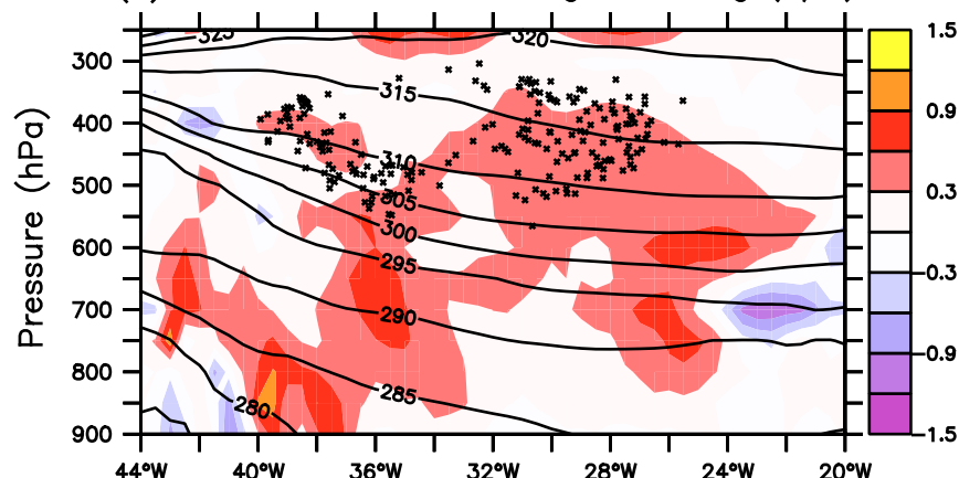
(f) NoConv, 63°N–65°N averaged heating (K/h)
