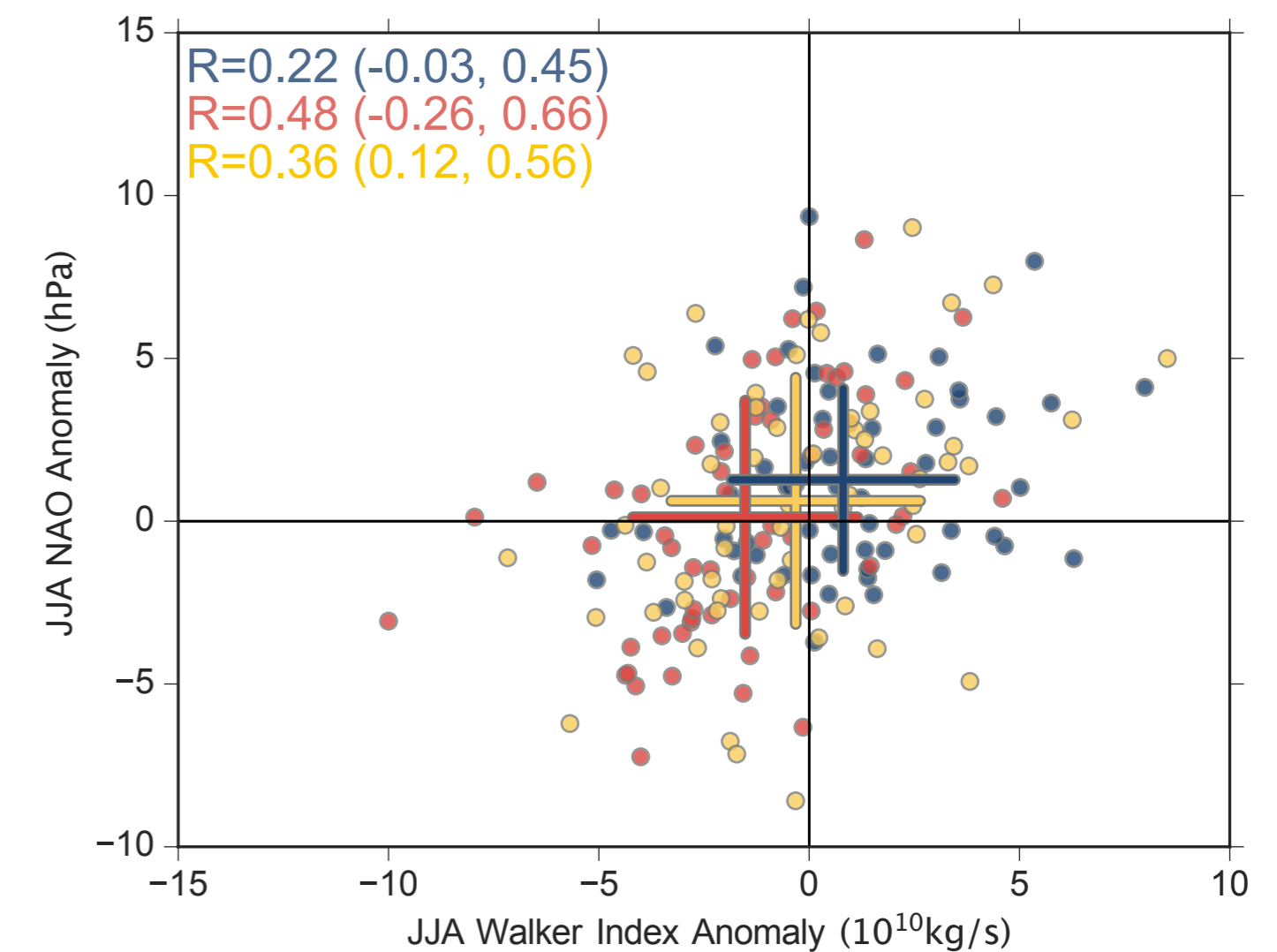
(f) JJA NAO vs. JJA Walker
