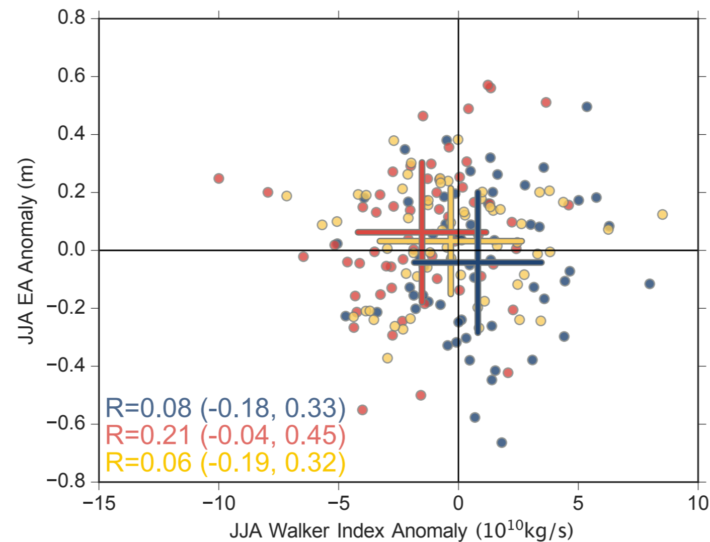
(e) JJA EA vs. JJA Walker
