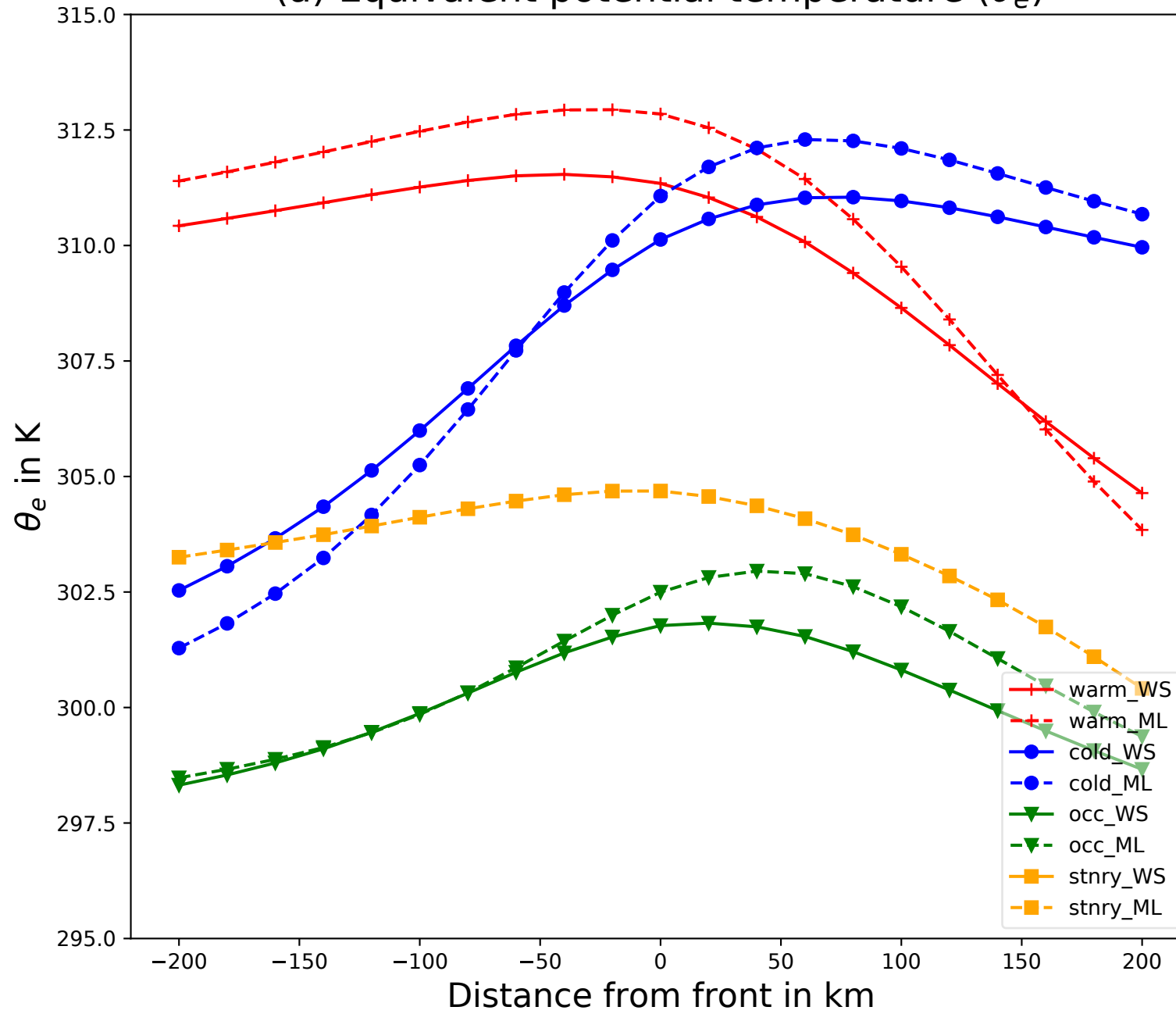
(a) Equivalent potential temperature ( \theta_e )
