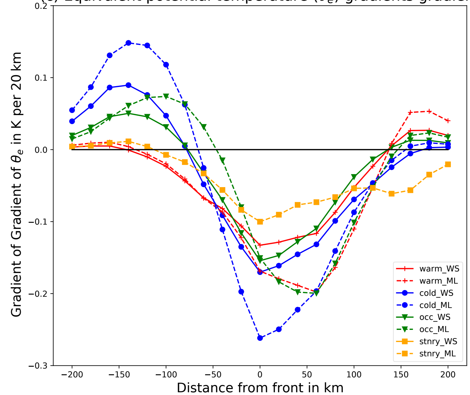
(c) Equivalent potential temperature ( \theta_e ) gradients gradient
