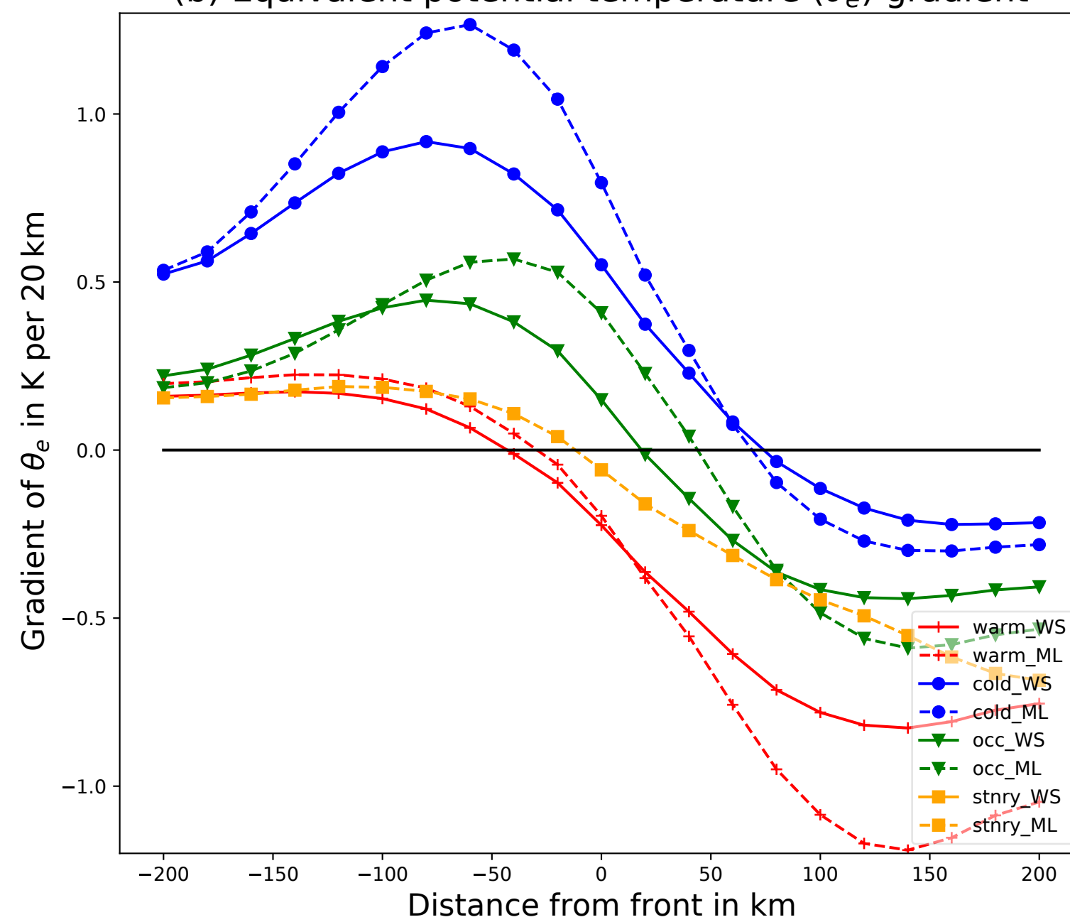
(b) Equivalent potential temperature ( \theta_e ) gradient
