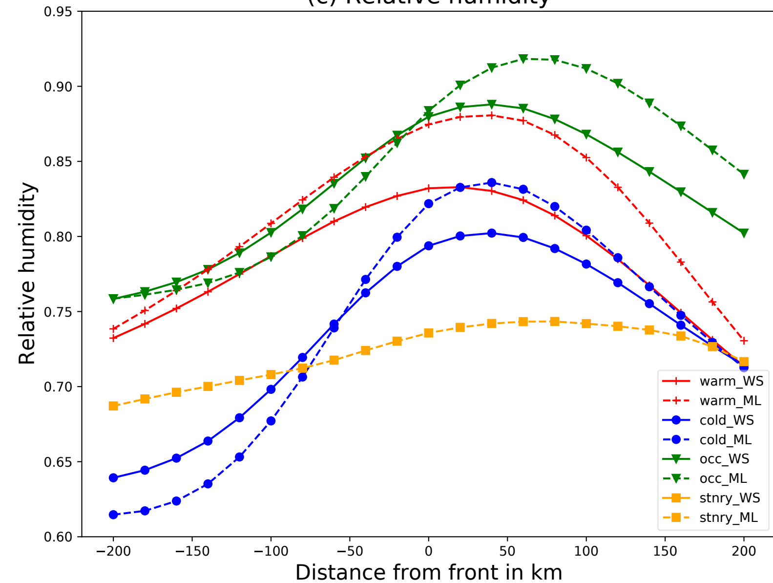
(c) Relative humidity
