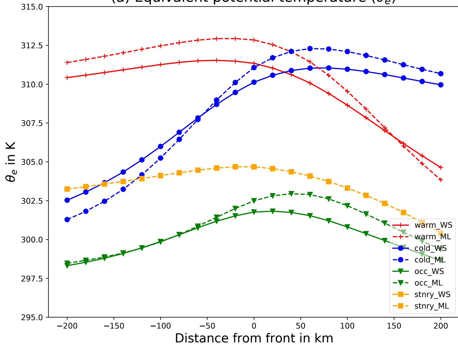
(a) Equivalent potential temperature ( \theta_e )
