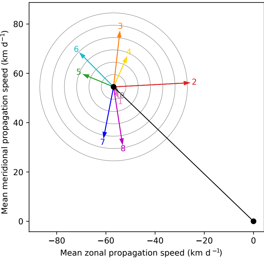
(a) LPSs north of 15°N
