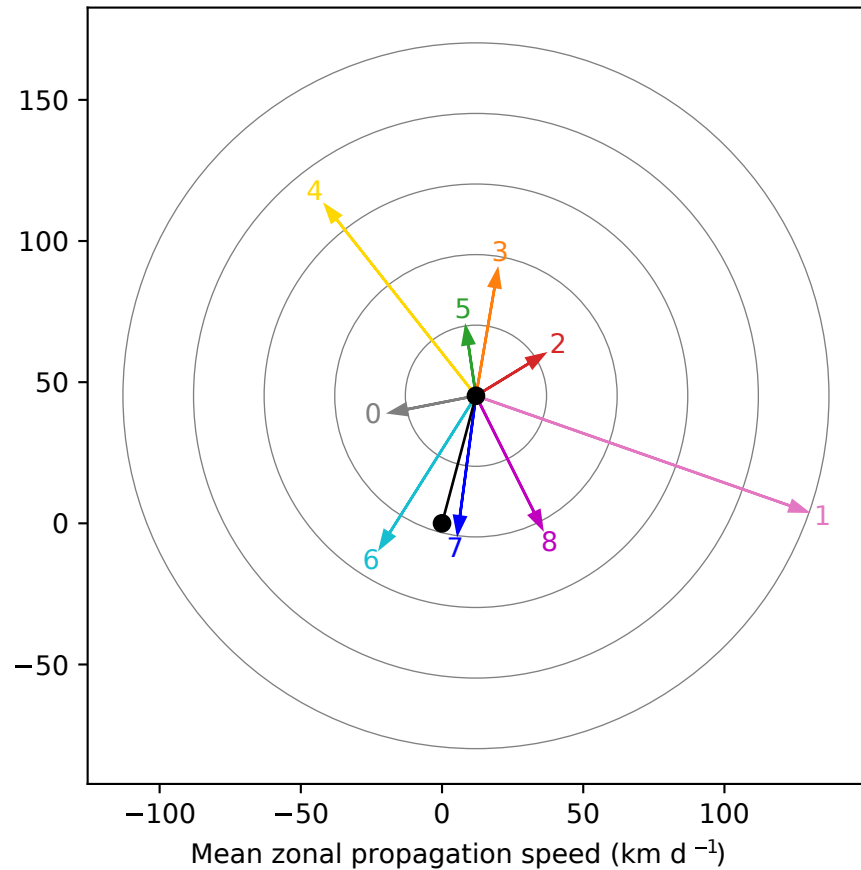
(b) LPSs south of 15°N
