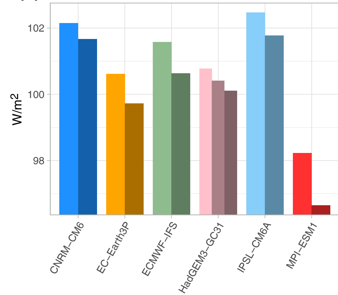
(c) Outgoing Shortwave Radiation
