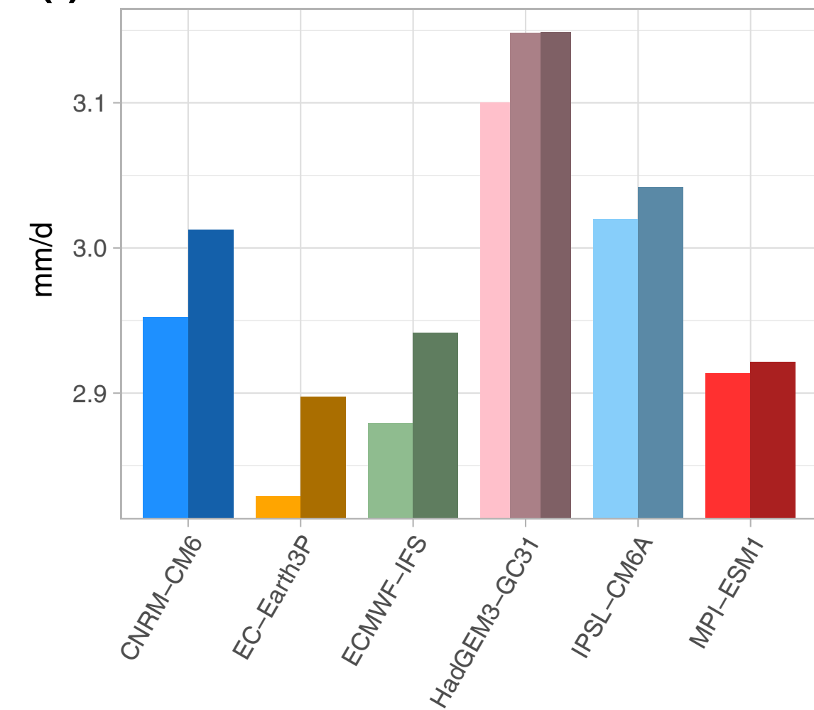
(f) Total Precipitation
