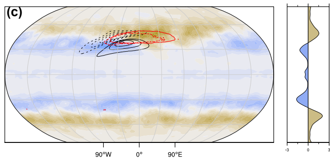
Change in barotropic conversion into EKE
