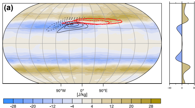
Change in EKE
