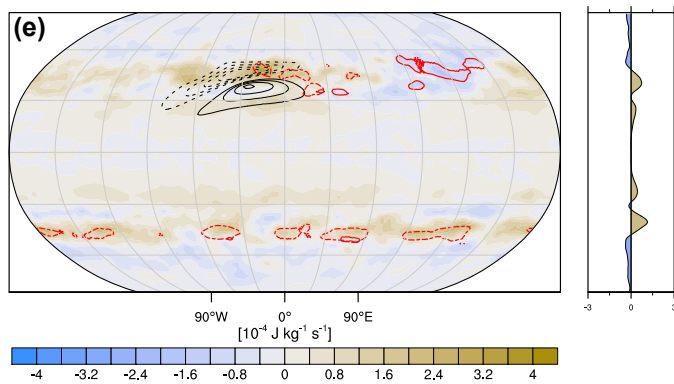
Change in barotropic conversion into EKE
