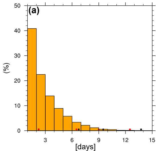
Lifetime (genesis near SST front)
