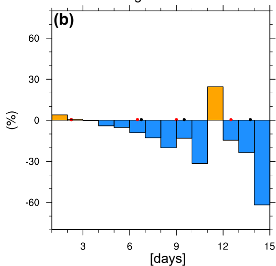
Relative change in warmer climate
