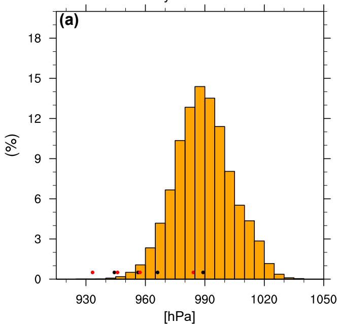
Maximum intensity (genesis near SST front)
