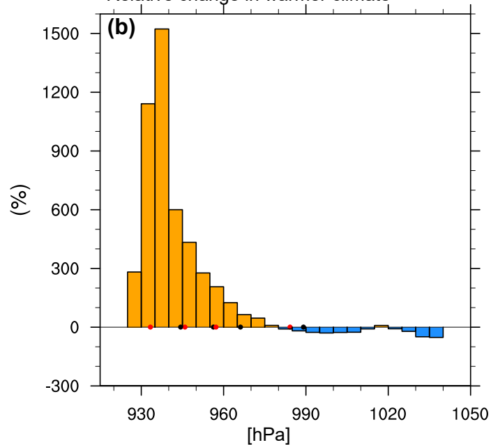
Relative change in warmer climate
