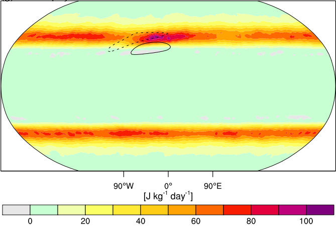
(g) Cloud physics at 700 hPa
