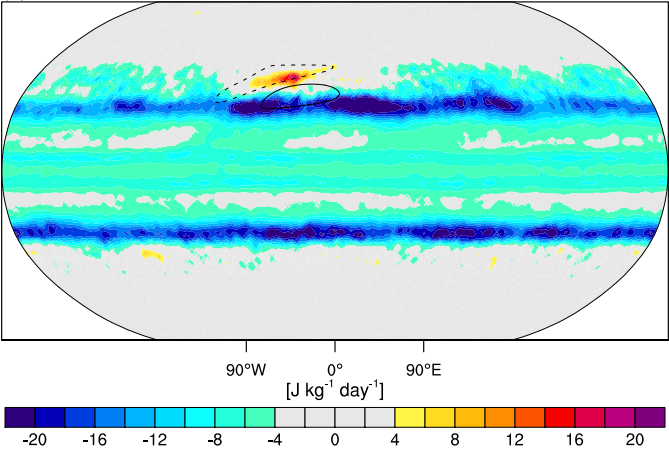
(b) Parameterized convection at 700 hPa
