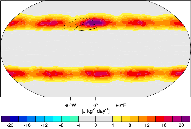
(e) Shortwave radiation at 300 hPa
