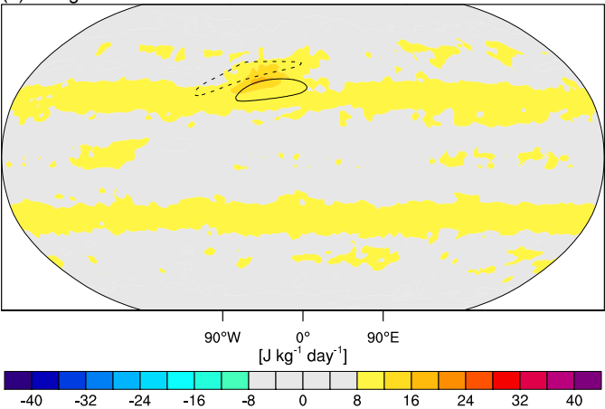
(f) Shortwave radiation at 700 hPa
