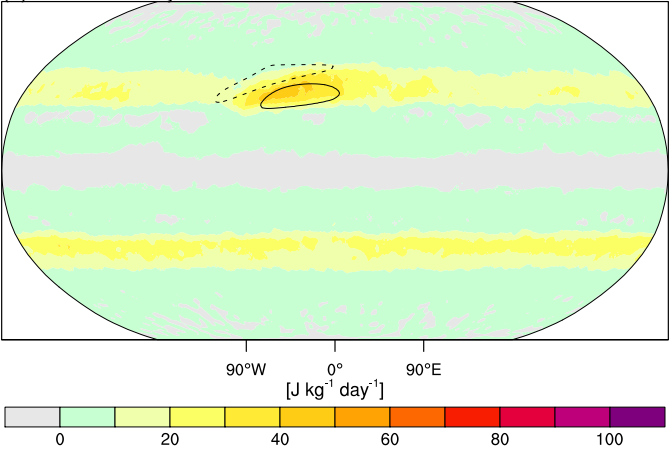
(h) Saturation adjustment at 700 hPa
