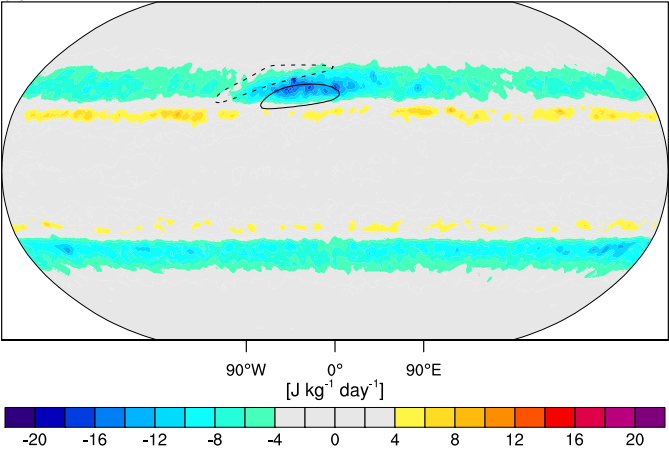
(a) Turbulence at 700 hPa
