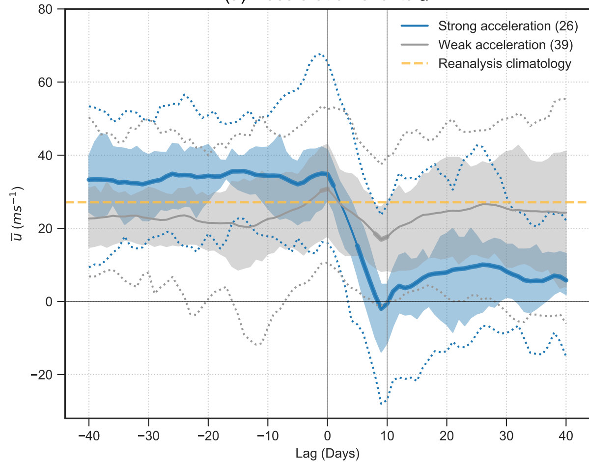
(a) Deceleration events \bar{u}
