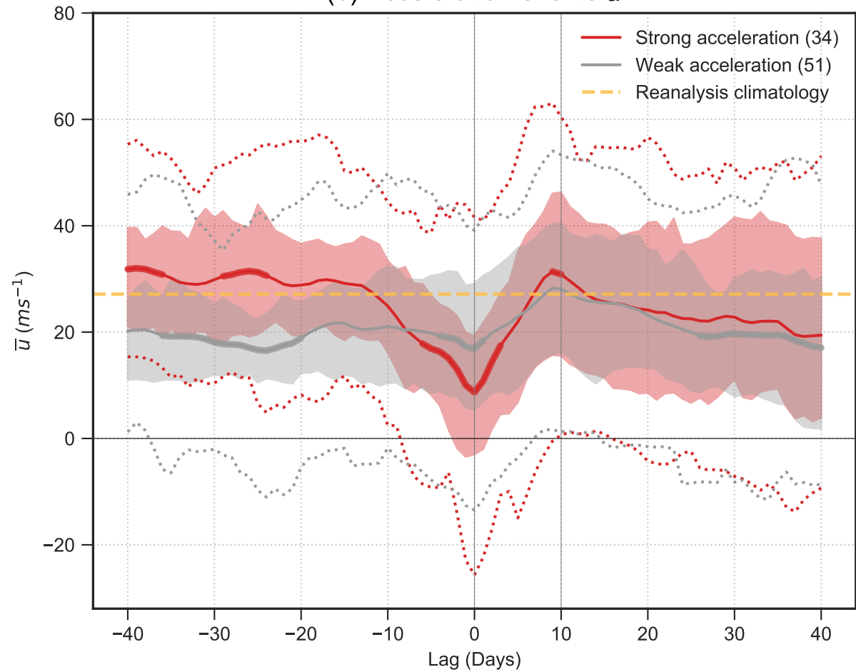
(b) Acceleration events \bar{u}
