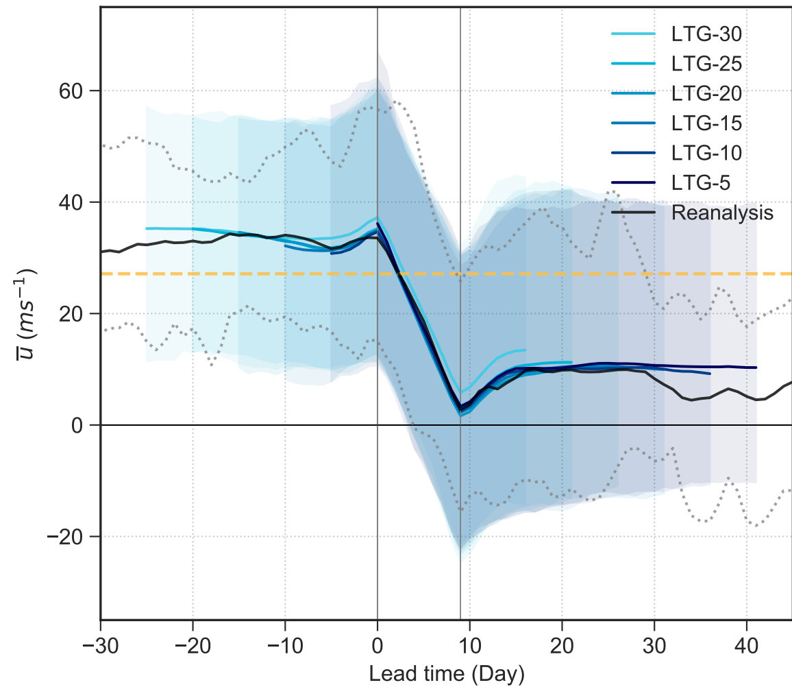
(a) Deceleration events \bar{u}
