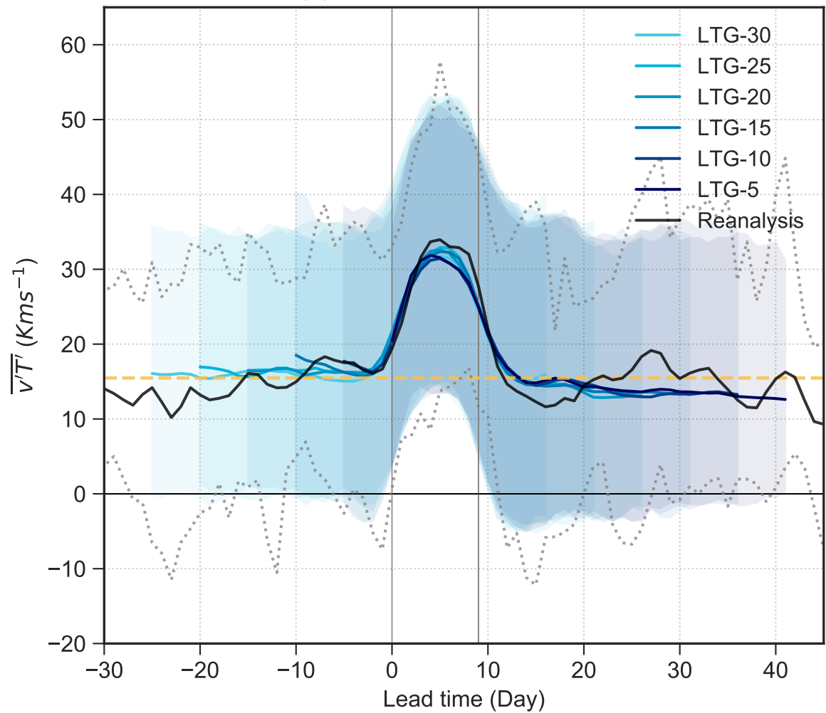
(b) Deceleration events \overline{v'T'}
