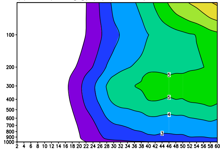
(c) Jan Spread [U](m/s) (60–90°N)
