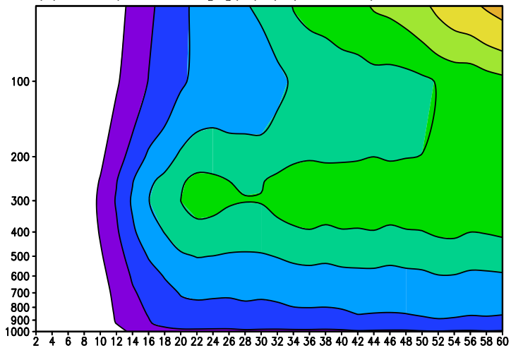
(a) Nov Spread T21 [U](m/s) (60–90°N)
