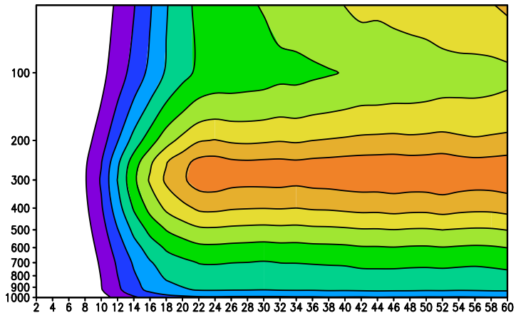
(b) Nov Spread T21 U(m/s) (m=1–3) (60–90°N)
