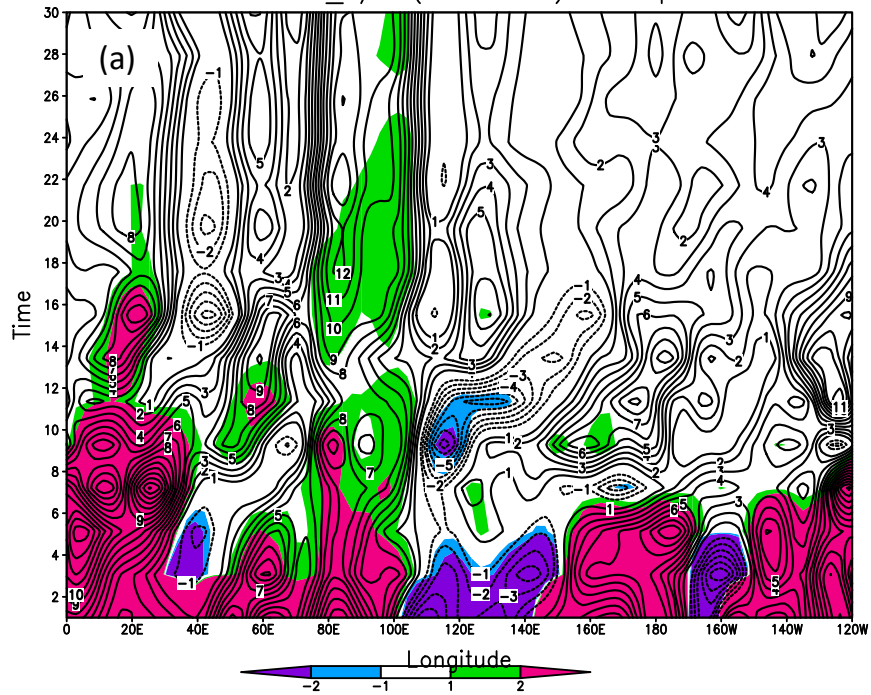
RWSDIV_s/n (20–35°N) All Exps
