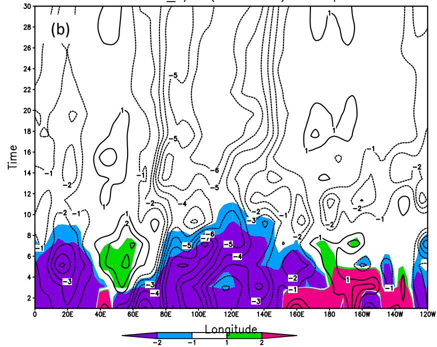
RWSADV_s/n (20–35°N) All Exps
