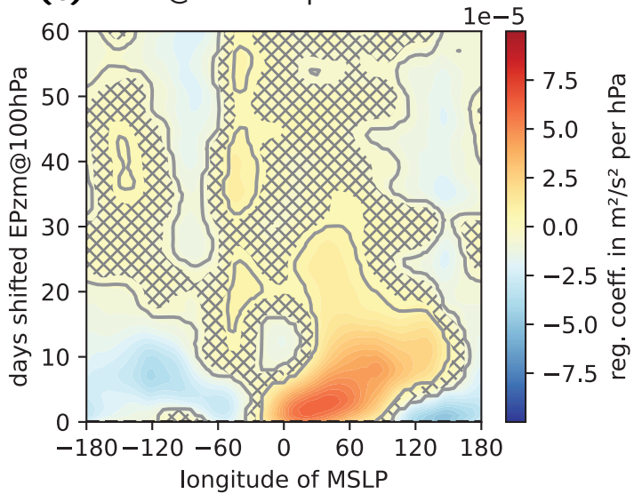
(b) EPzm@100hPa per MSLP
