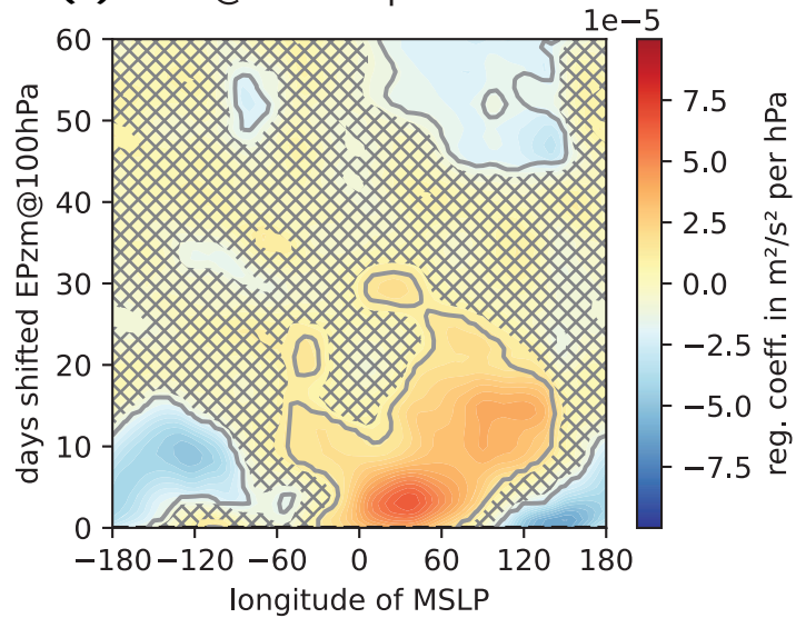
(a) EPzm@100hPa per MSLP
