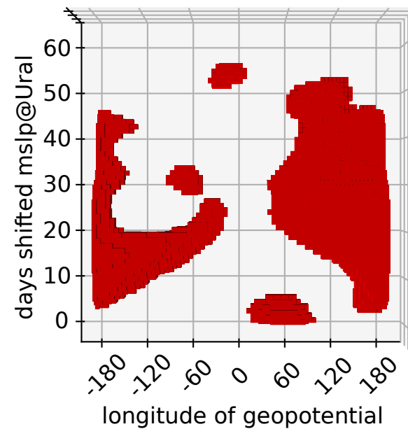
(c) top view stratosphere 100–1 hPa
