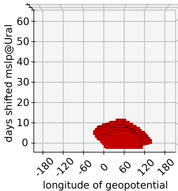
(b) top view troposphere 1000–200 hPa
