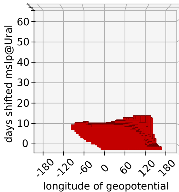
(e) top view troposphere 1000–200 hPa
