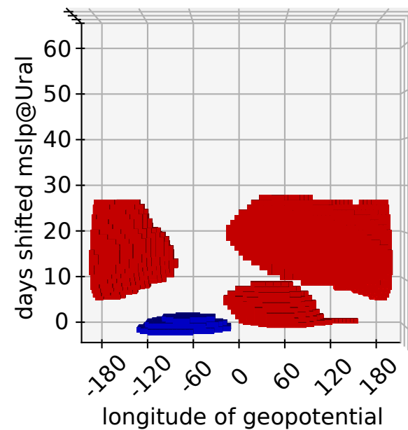
(f) top view stratosphere 100–1 hPa
