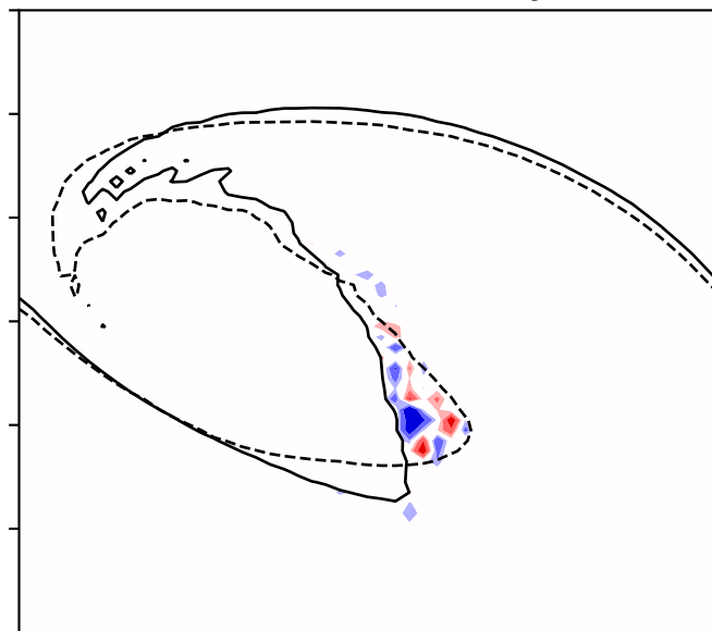
(b) Diabatic tendency
