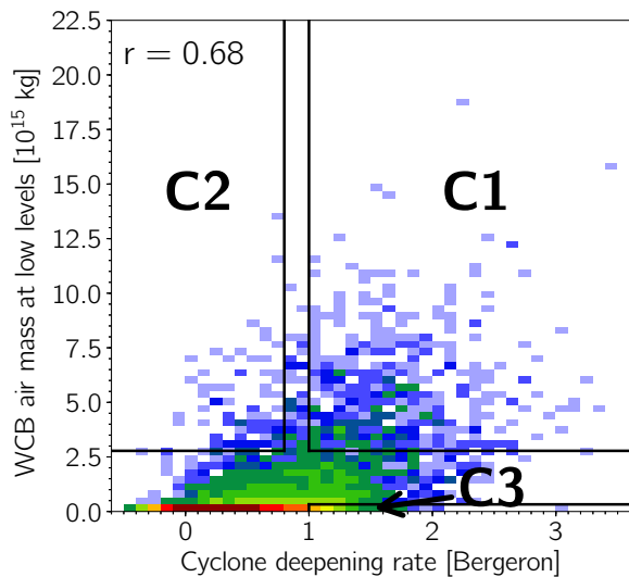
(c) CESM-HIST, NH
