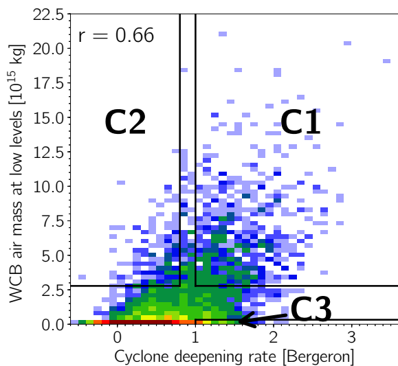
(e) CESM-RCP85, NH
