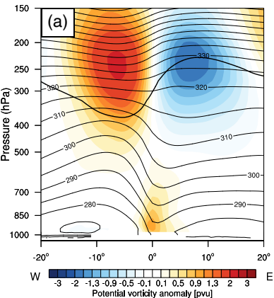
CESM-HIST, SH
