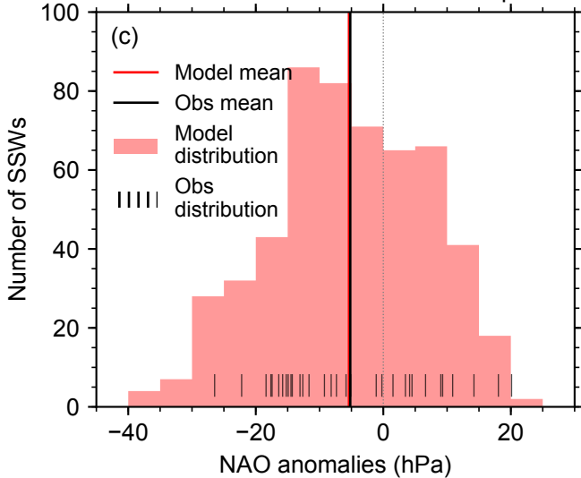
Distributions of individual 30d NAO responses
