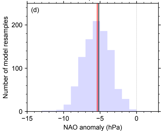
Mean 30d NAO responses over all SSWs
