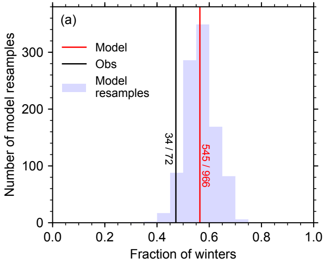
Fraction of winters with at least one SSW
