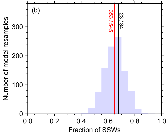
Fraction of SSWs with NAO – responses
