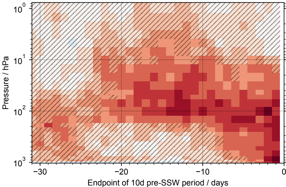
Difference between probabilities of negative NAO when subset by terciles of 60°N ZMW (lower minus upper)
