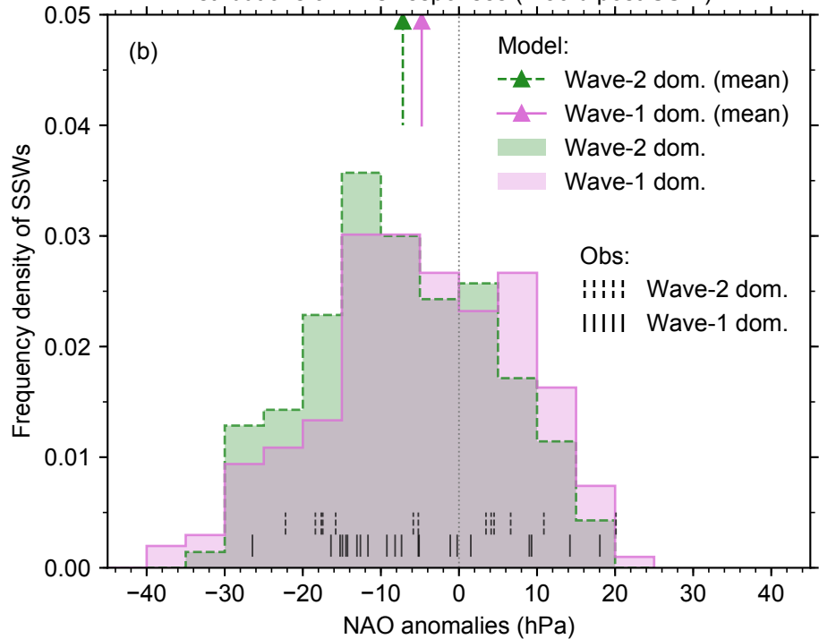
Distributions of NAO responses (1-30 d post-SSW)
