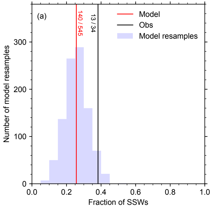
Fraction of SSWs that are wave-2 dominated
