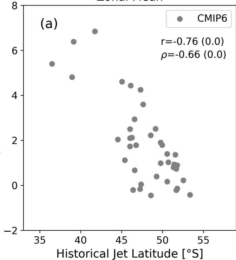
Zonal Mean
