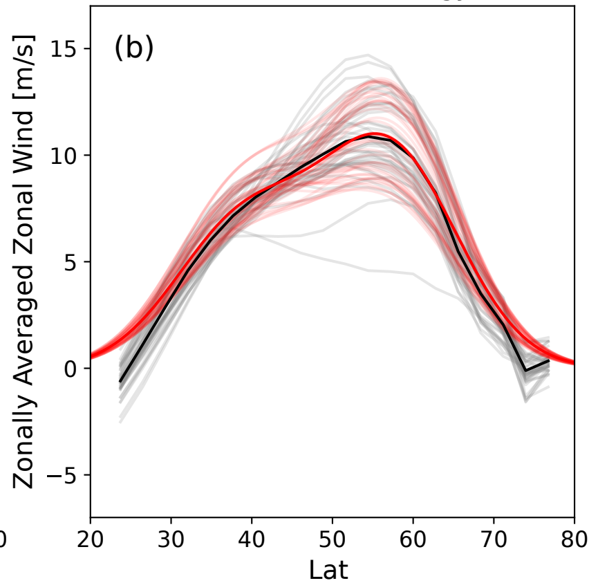
SSP5-8.5 Climatology
