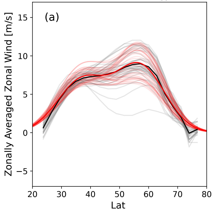
Historical Climatology
