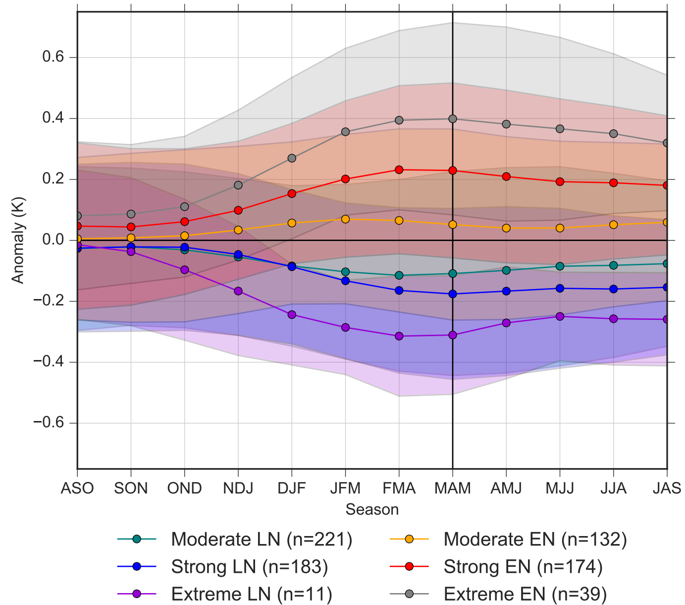
(b) TNA SSTA Evolution (FOCI)
