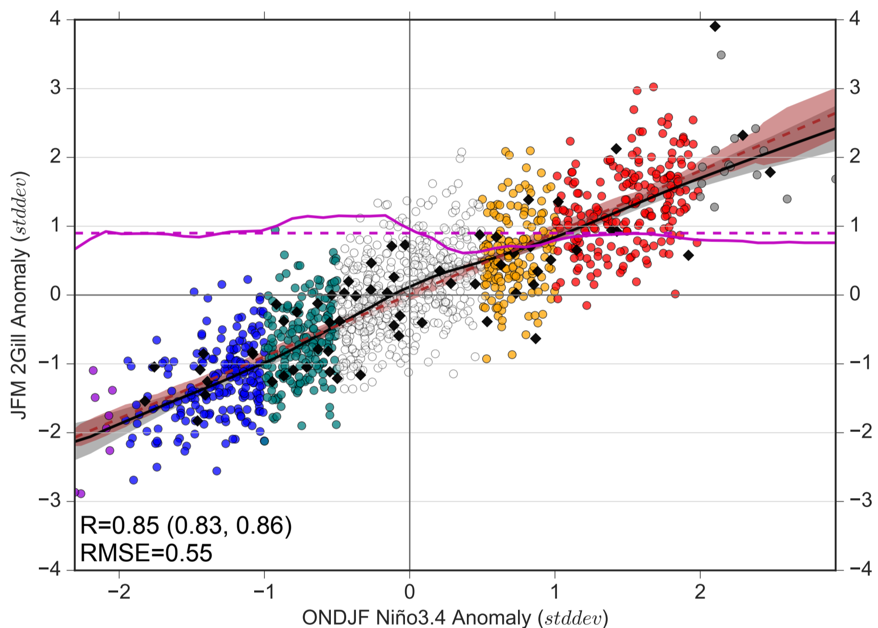
(e) Southeastern Low Response (CESM-WACCM)
