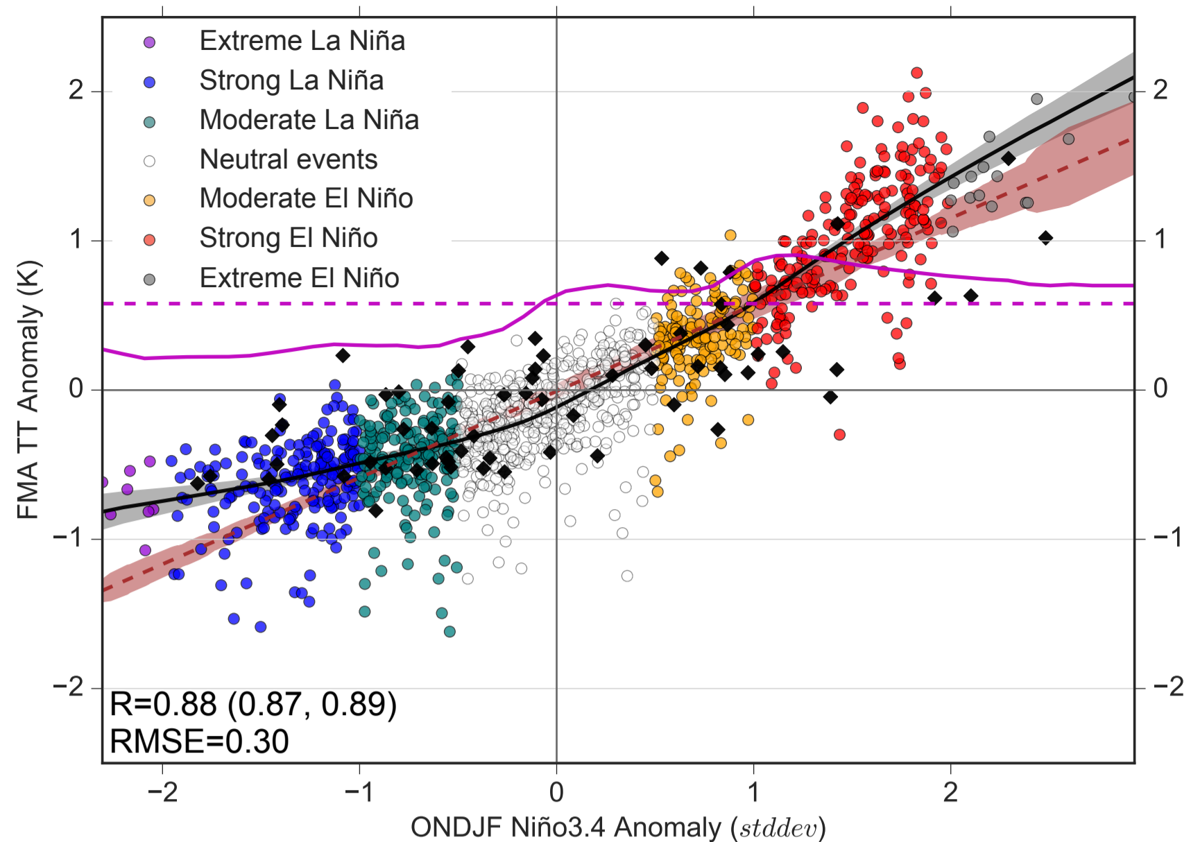
(c) Secondary Gill Response (CESM-WACCM)
