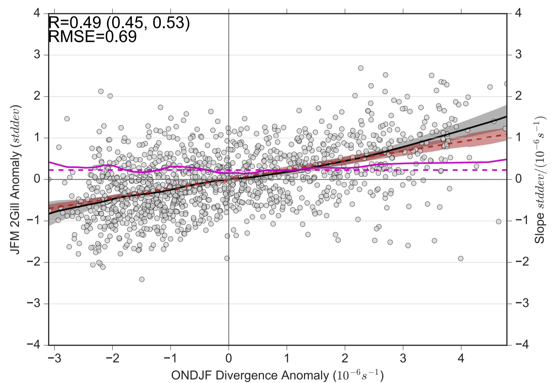
(f) FOCI SEL vs. 200 div. (166°E-158°W)
