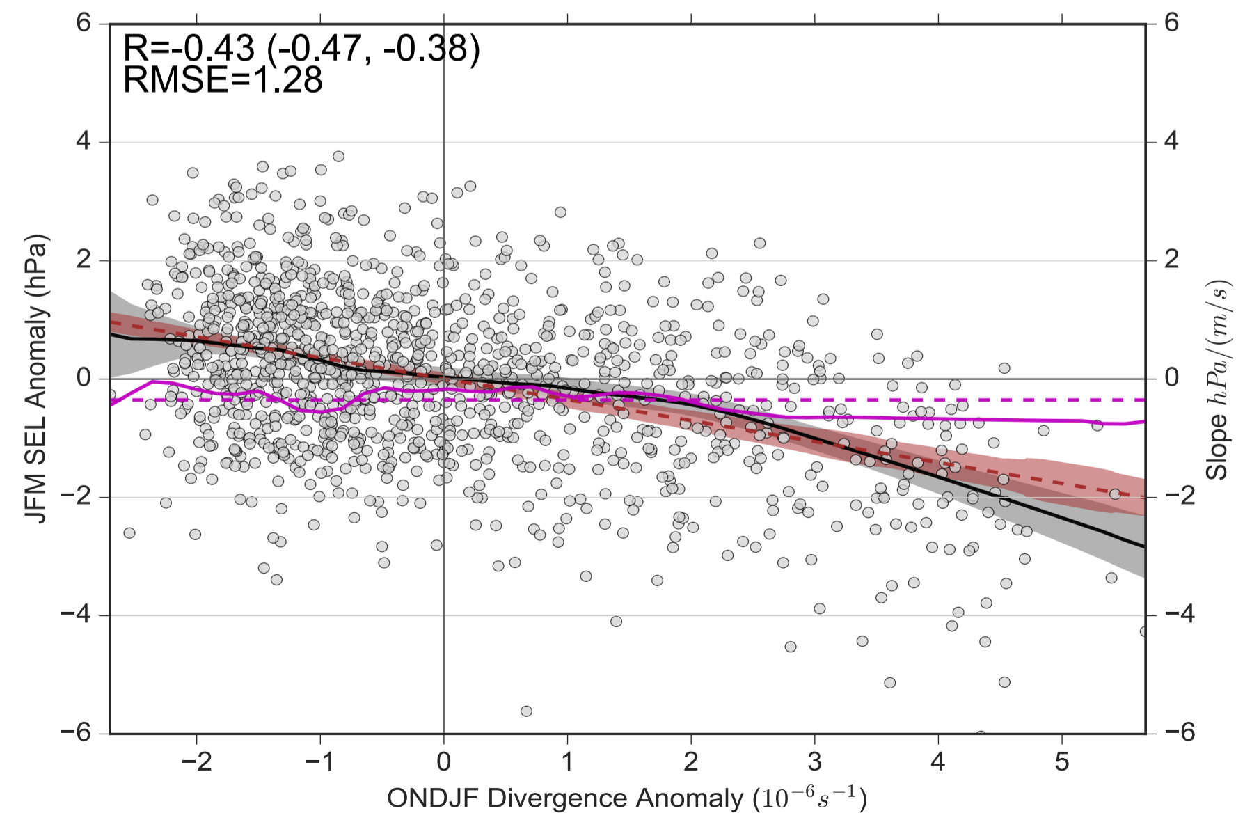
(f) FOCI SEL vs. 200 div. (166°E-158°W)
