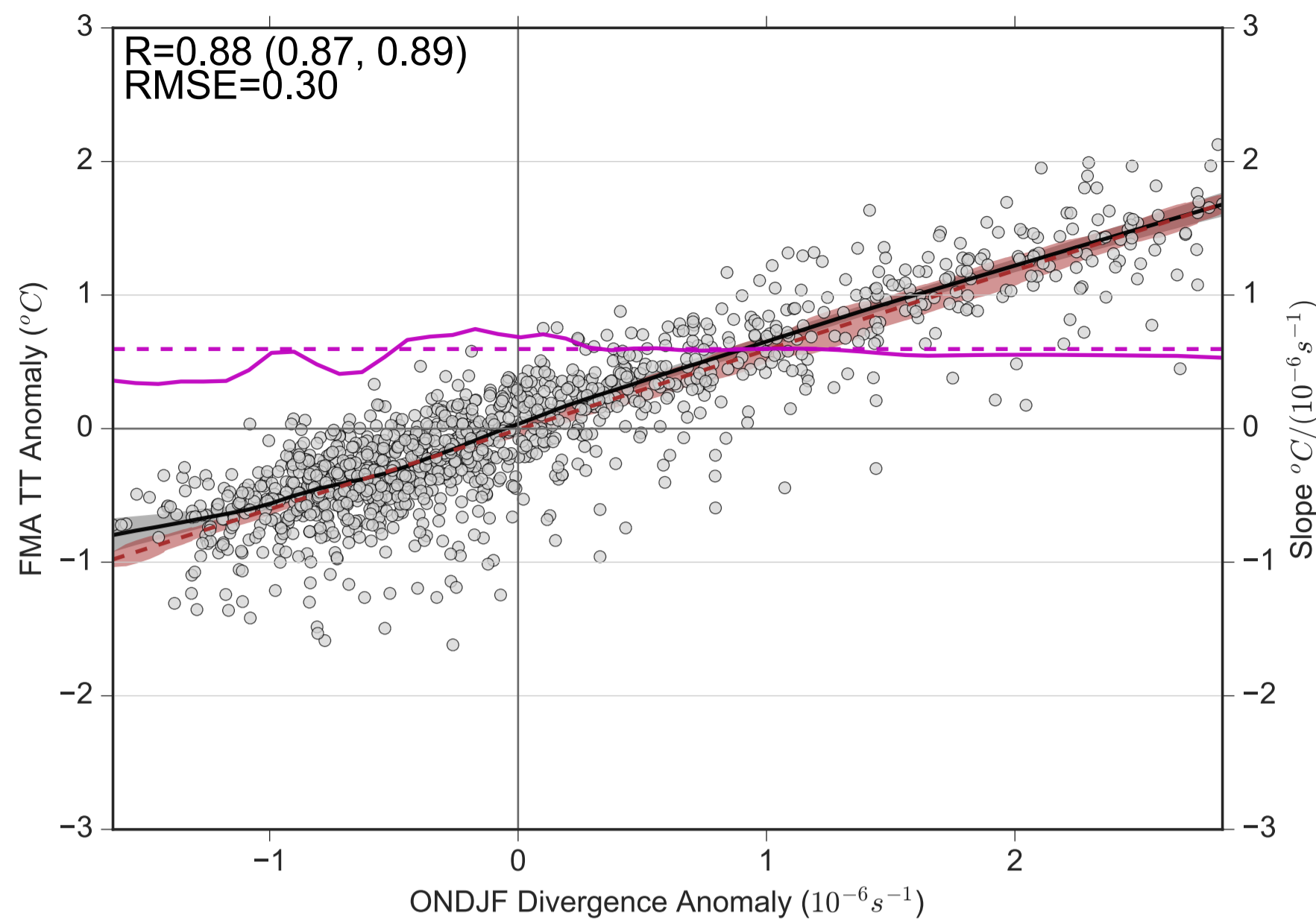
(c) CESM-WACCM 2Gill vs. 200 div. (130°E-115°W)
