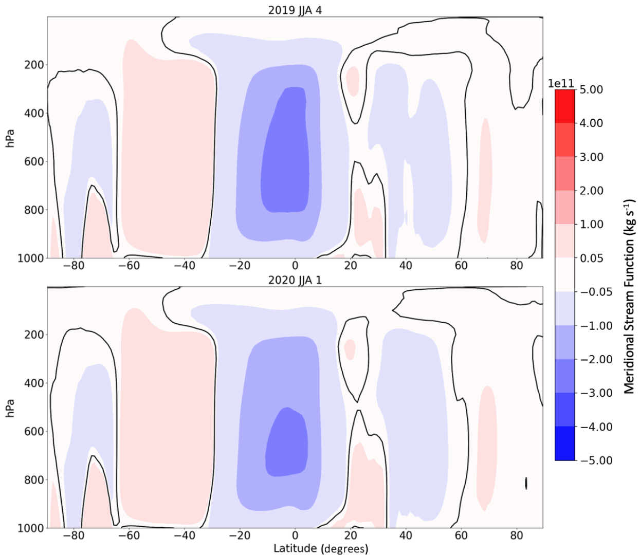
40 Fig. S1: SF values ( \text{kg s}^{-1} ) for ensemble member 4 in JJA 2019, and ensemble member 1 in JJA 2020, showing an unenclosed NH HC. The black contours indicate the zero-crossing, while shading signifies SF intensity. Note the region near 500 hPa and 20 degrees in both years where there is no positive circulation.
