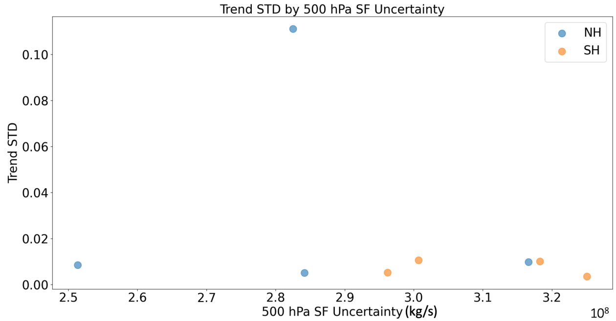
100 Fig. S5: SF trend STD (degrees per decade) by 500 hPa SF uncertainty ( \text{kg s}^{-1} ) for all four seasons in both hemispheres.
