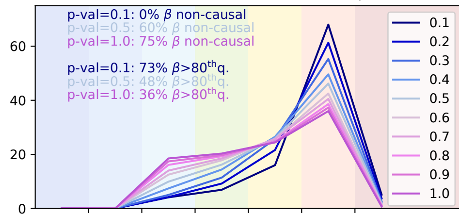
(h) All links, MCA2 WNPSM \Rightarrow OLR|NPH
