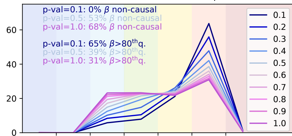
(f) All links, MCA2 WNPSM \Rightarrow Z200|NPH
