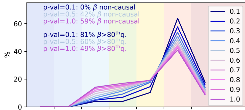
(c) All links, MCA1 CGT \Rightarrow OLR|SAM
