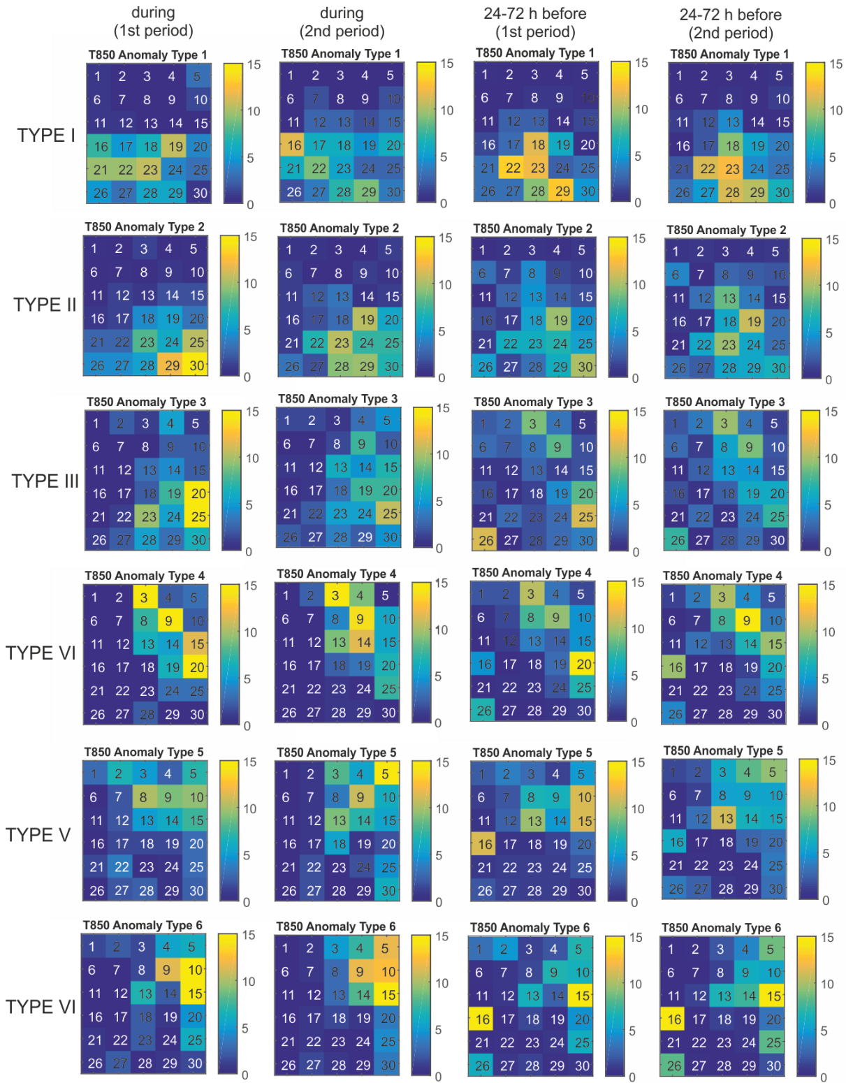
Figure S7. Relative distribution of circulation types during (two columns on the left) and 24–72 h before the start of (two column on the right) the six cold anomaly types. Results for 1979–1999 (first period) and 2000–2020 (second period) are shown separately. Numbers (1–30) refer to MSLP SOM node numbers in Fig. 3 (and in 500 hPa geopotential SOM composite in Supplementary Fig. 4).
