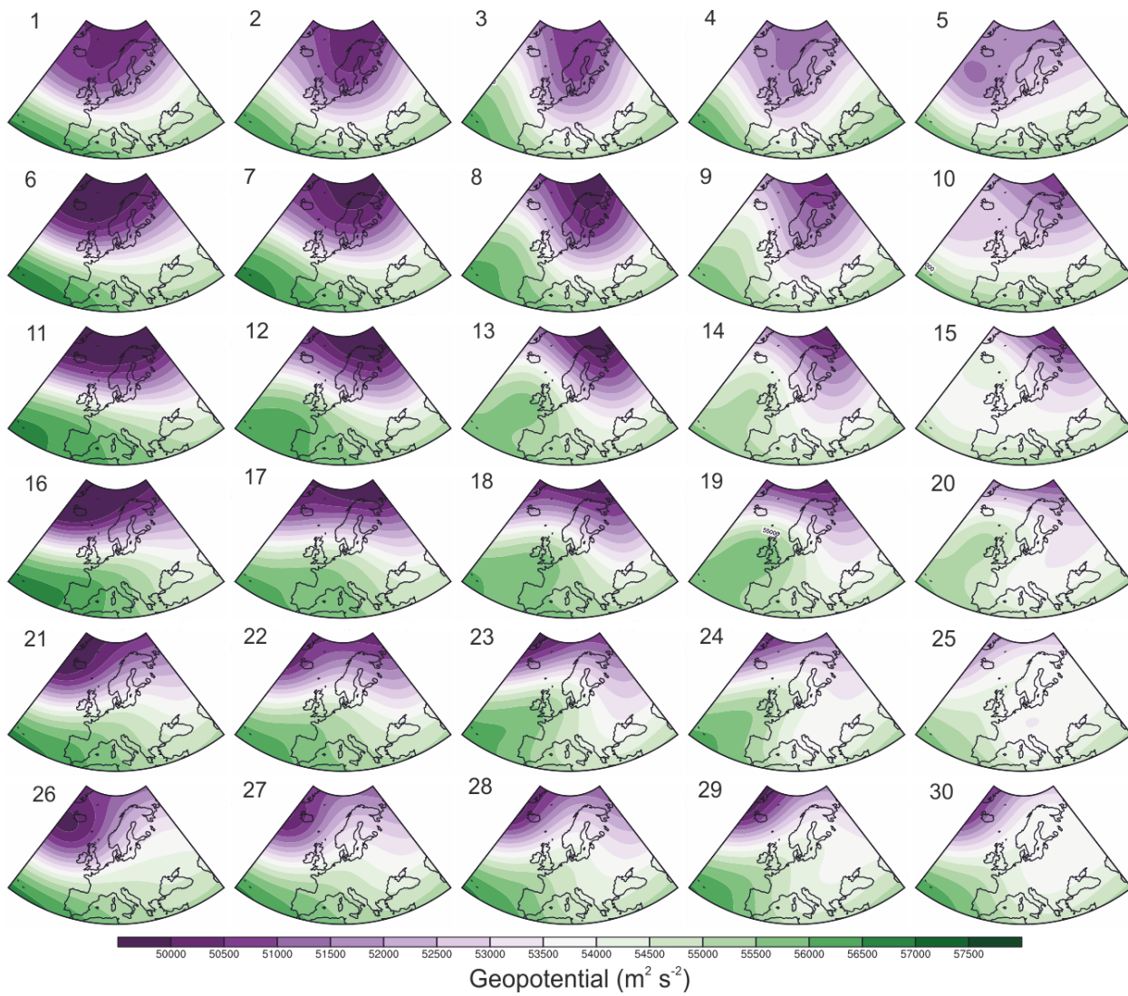
Figure S4. A 5 x 6 SOM composite array of daily mean 500 hPa geopotential in November–March 1979–2020.
