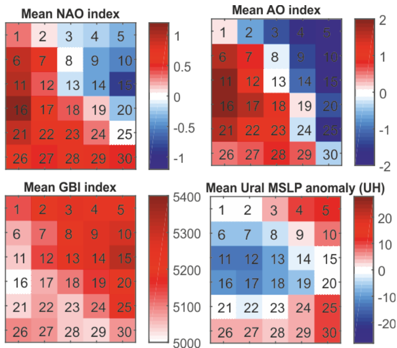
Figure S5. Mean NAO (left top), AO (right top), GBI index (left down) and mean Ural MSLP anomaly, representing UH, (right down) linked to MSLP (and 500 hPa geopotential) SOM patterns. Numbers (1–30) refer to MSLP SOM node numbers in Supplementary Fig. 3 (and to 500 hPa geopotential SOM composite in Supplementary Fig. 4).
