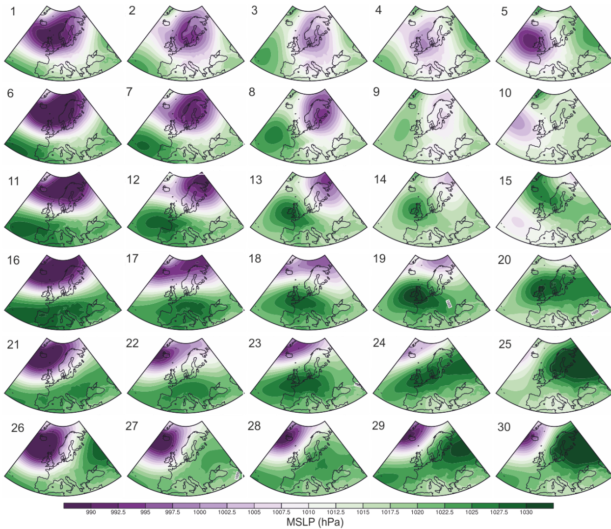
Figure S3. A 5 x 6 SOM composite array of daily mean sea level pressure in November–March 1979–2020.
