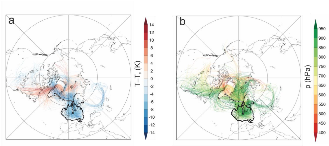
Figure S6. (a) Evolution of the temperature anomaly ( T-T_c ), and (b) pressure along backward trajectories (10 days) associated with a cold anomaly event on 31 March 1996 (cold anomaly Type IV). The region indicated by a black line is the cold anomaly region (where 850 hPa temperature was lower than the 10 th percentile) of this event. Trajectory ensemble end points are at the 850 hPa level in the marked cold anomaly region. The end point regions were determined for each individual case separately, by taking the area with 850 hPa temperature being lower than the 10 th percentile. The centroid trajectory is marked with a thick line and black dots indicate the air parcel position in daily intervals.
