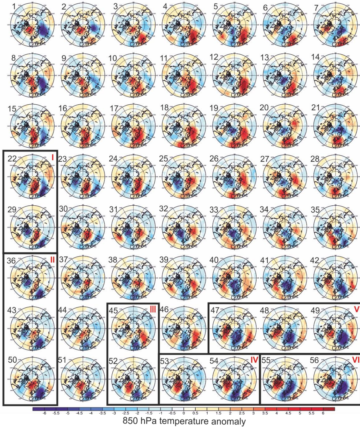
Figure S2. 2 A 7 x 8 SOM composite array of daily 850 hPa temperature anomalies in November–March 1979–2020 over the circumpolar region north of 35°N. Note that the SOM analysis is only made for Europe (see the region in Fig. 2). Anomalies outside Europe thus indicate connections with anomalies over Europe. The six cold anomaly types (I–VI) of Europe are marked.
