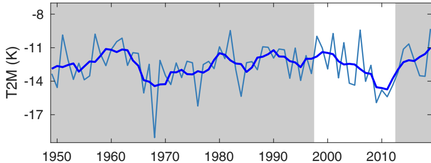
(a) Eurasian DJF temperature
