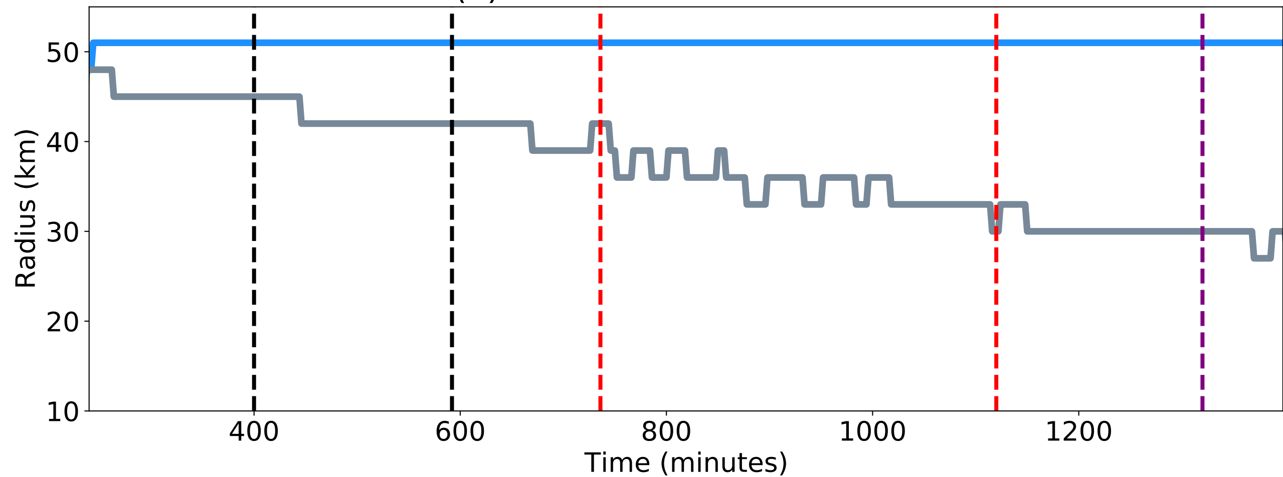
(b) Radius of Maximum Wind
