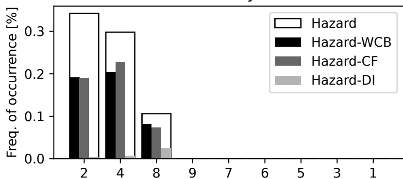
pm10-Heat and Dyn. Features
