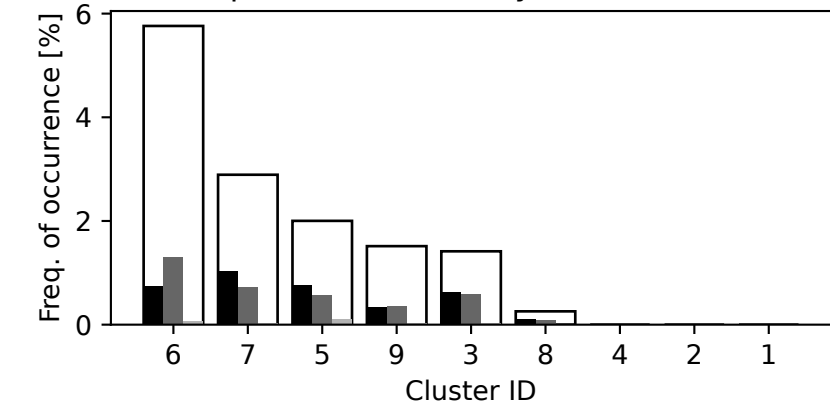
pm10-Heat and Dyn. Features
