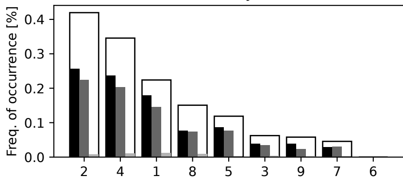
Rain-Wave and Dyn. Features
