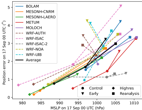
(a) Link between position and intensity of Ianos
