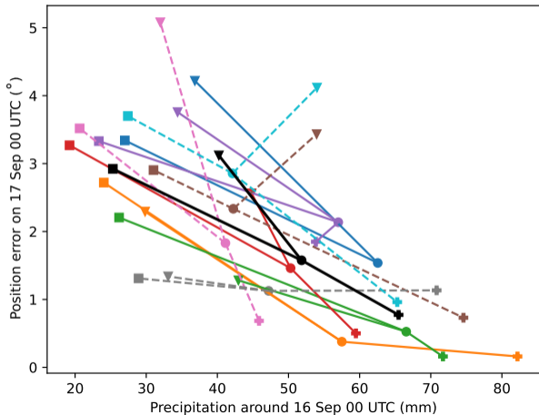
(b) Link between position and precipitation of Ianos
