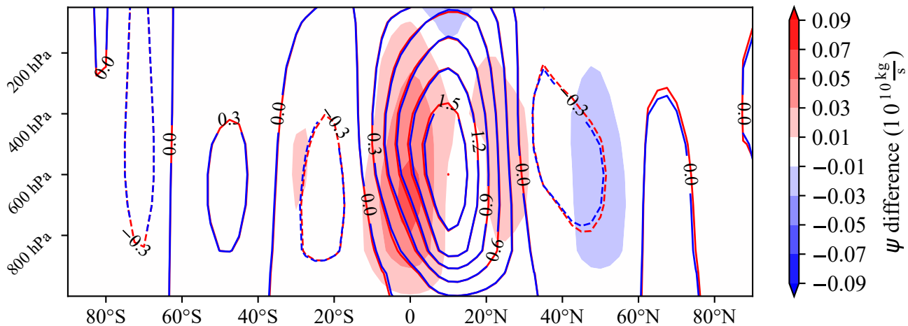
(b) Mass overturning streamfunction in the meridional plane
