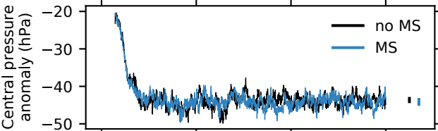
(c) Half-earth-radius TC world
