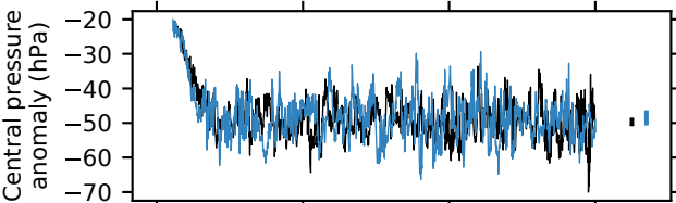
(e) Quarter-earth-radius TC world
