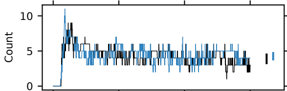
(f) Quarter-earth-radius TC world
