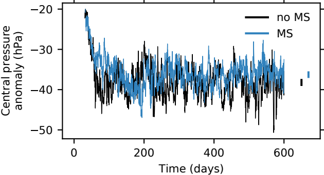
(e) Quarter-earth-radius TC world
