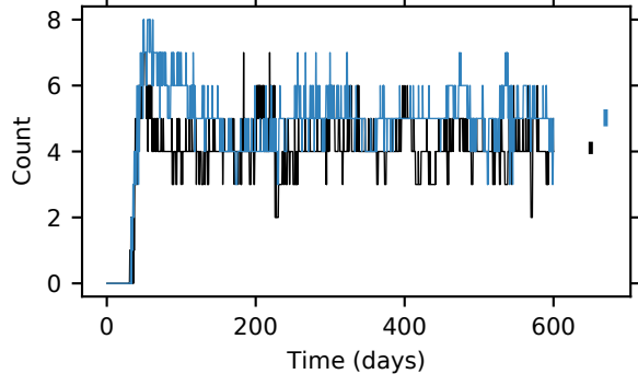
(b) Quarter-earth-radius TC world
