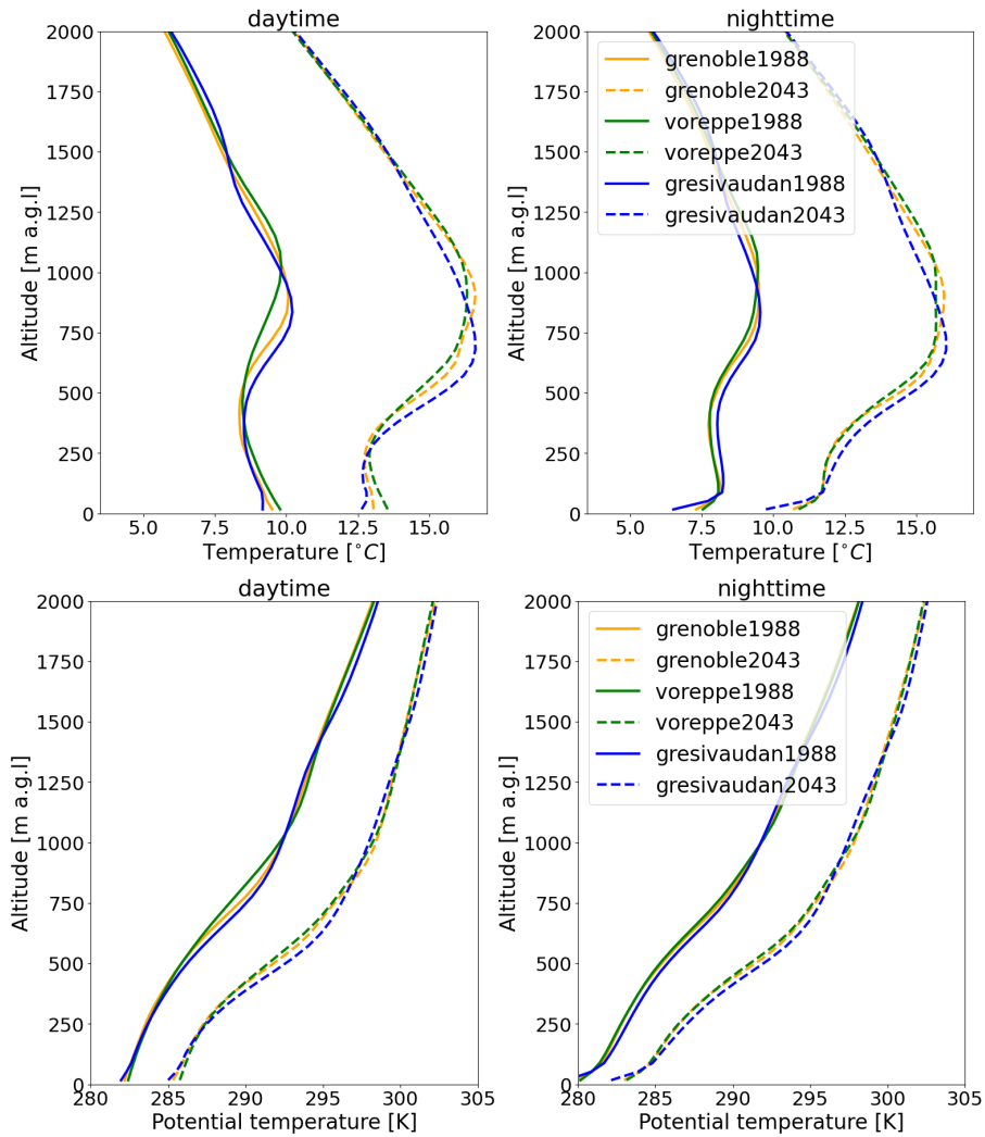
Figure S9: Vertical profiles of temperature (upper row) and potential temperature (bottom row) during daytime (left) and nighttime (right) spatially averaged over the Grenoble basin (orange), Voreppe valley (green) and Grésivaudan valley (blue) for Ep1988 (continuous line) and Ep2043 (dashed line). The daytime (nighttime) is defined between 8:00 UTC and 18:00 UTC (18:00 UTC and 8:00 UTC). Each profile is also averaged over the three selected days and nights of each episode, which are 18-20 December 1988 and 8-10 December 2043.
