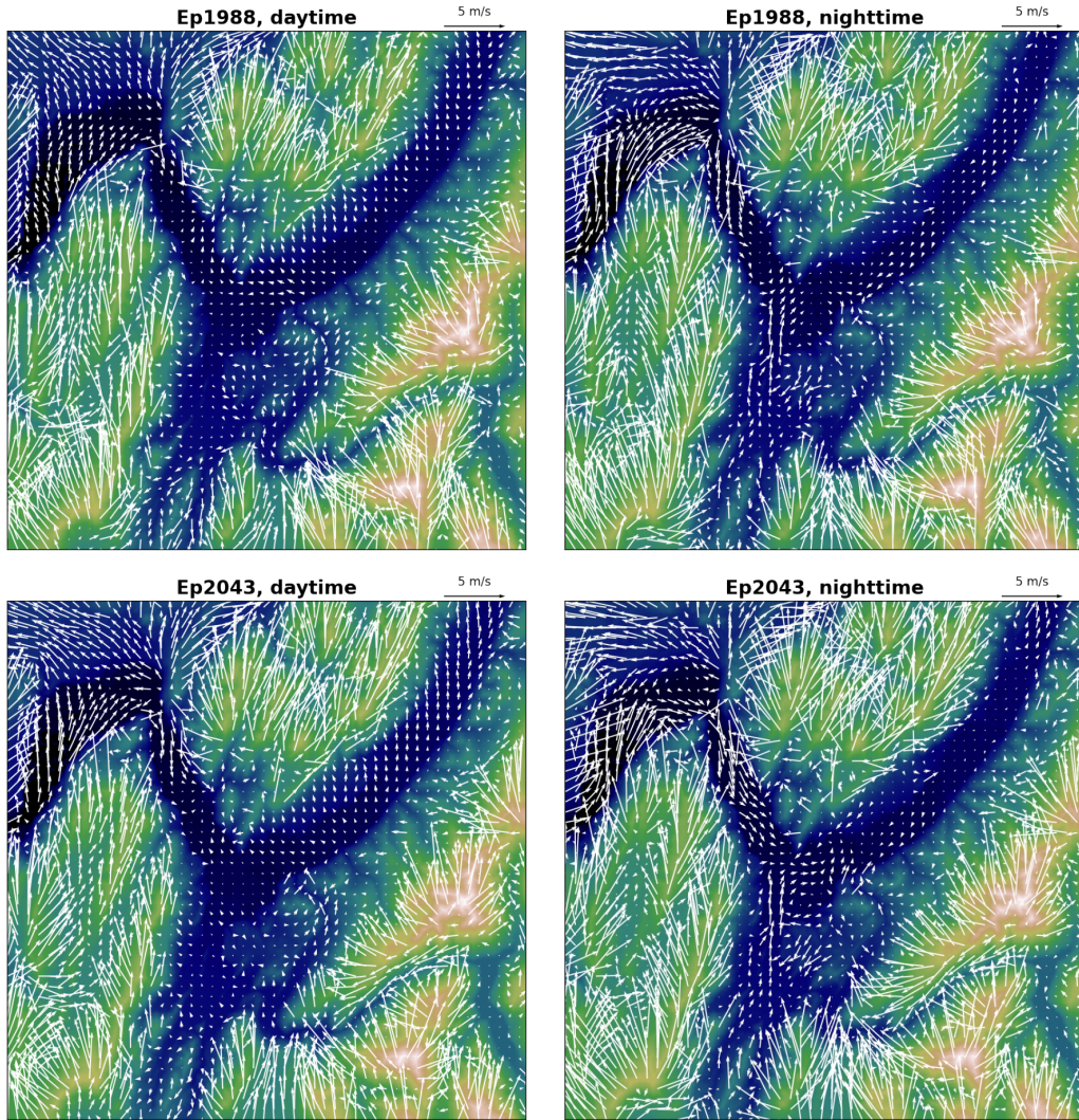
Figure S10: Horizontal wind at 10 m a.g.l. for daytime and nighttime of Ep1988 and Ep2043. The winds are temporally averaged for daytime (from 8:00 UTC to 18:00 UTC) and nighttime (from 18:00 UTC to 8:00 UTC) for the three selected days of the episodes.
