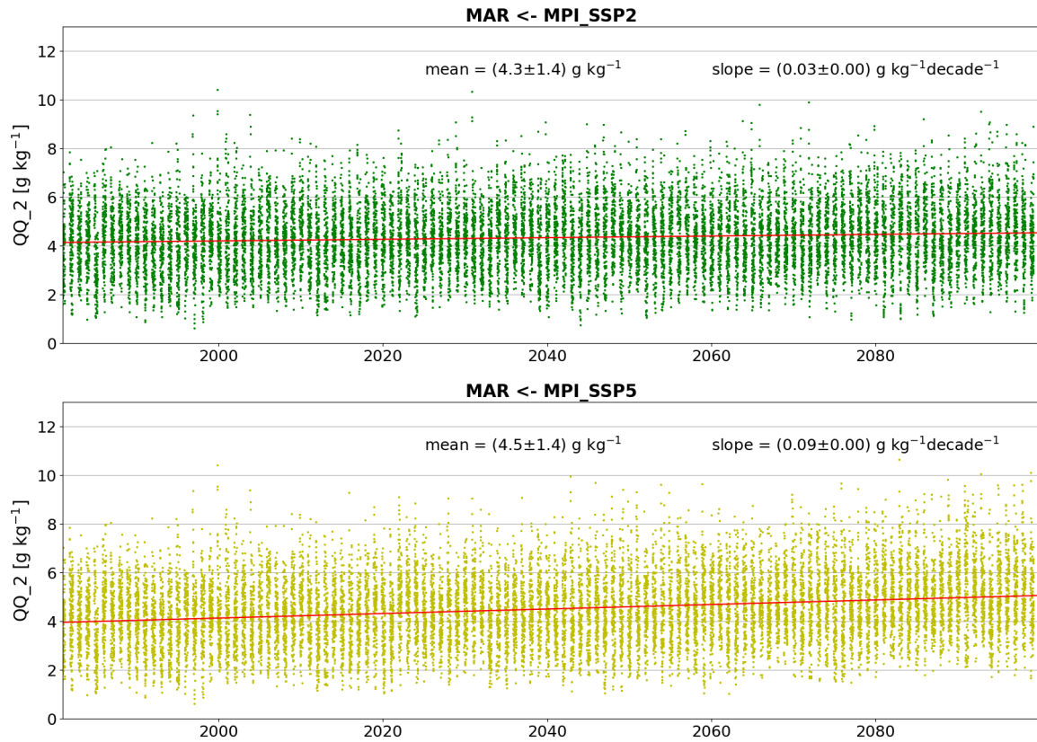
Figure S6: Temporal series of daily winter specific humidity at 2m above the ground for MAR←MPI_SSP2 (upper row) and MAR←MPI_SSP5 (bottom row) at the GR grid box. The red line is the trend (which is statistically significant at 95%). The mean and the slope of the trend refer to the entire time series (i.e. 120 winters).
