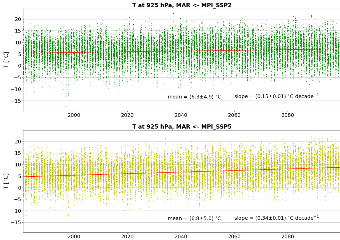
Figure S5: Temporal series of daily winter temperature at 925 hPa ( T_{925\text{hPa}} ) for MAR←MPI_SSP2 (upper row) and MAR←MPI_SSP5 (bottom row) at the GR grid box. The red line is the trend (which is statistically significant at 95%). The mean and the slope of the trend refer to the entire time series (i.e. 120 winters).
