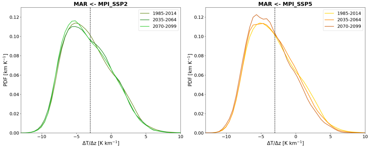
Figure S3: Normalized probability density functions (PDFs) of daily (\Delta T/\Delta z)_{\text{MAR}} computed with MAR←MPI_SSP2 and MAR←MPI_SSP5 for 30 years around 2000, 2050, and 2085 during NDJFM. The vertical line is at \Delta T/\Delta z = -3 \text{ K km}^{-1} (i.e. the threshold used to identify PCAP episodes).
