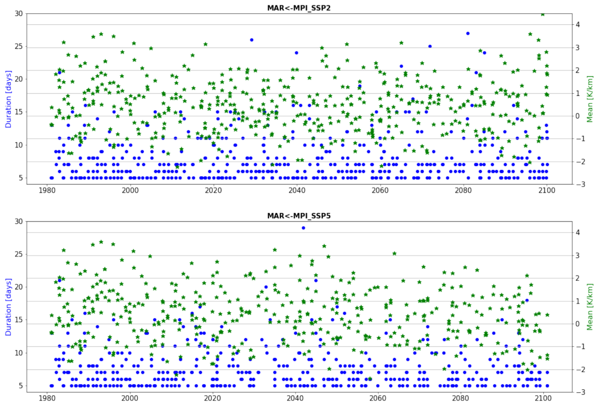
Figure S7: Duration (blue) and intensity (green) of all PCAP episodes identified by MAR←MPI_SSP2 and MAR←MPI_SSP5.
