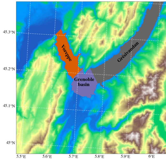
Figure S8: Areas considered for the spatially-averaged fields in section 5.2.
