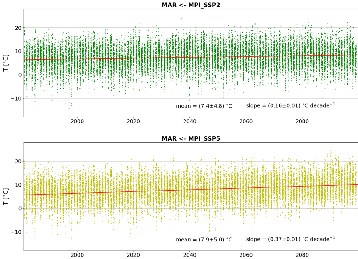
Figure S4: Temporal series of daily winter temperature at 2 m ( T_{2\text{m}} ) for MAR←MPI_SSP2 (upper row) and MAR←MPI_SSP5 (bottom row) at the GR grid box (see section 2.2.2 for the definition of this point). The red line is the trend (which is statistically significant at 95%). The mean and the slope of the trend refer to the entire time series (i.e. 120 winters).
