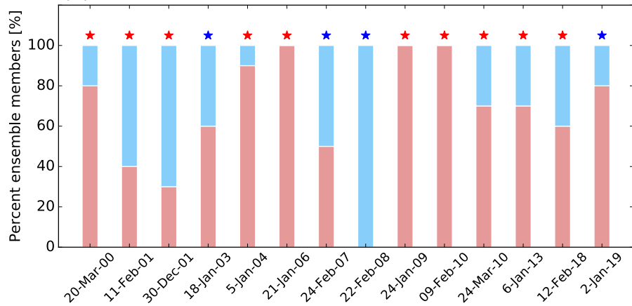
(c) Strong vortex events
