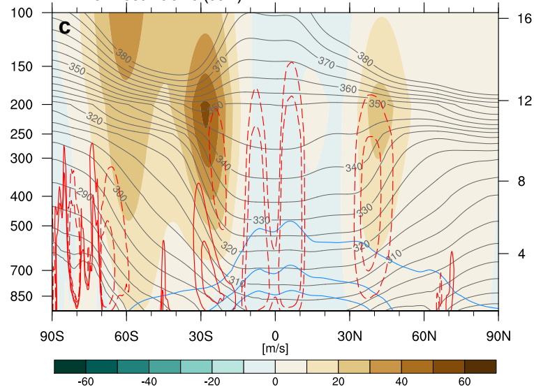
ERA5 West Pacific (JJA)
