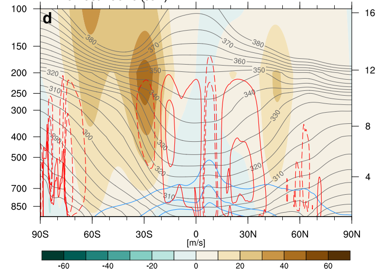
ERA5 East Pacific (JJA)
