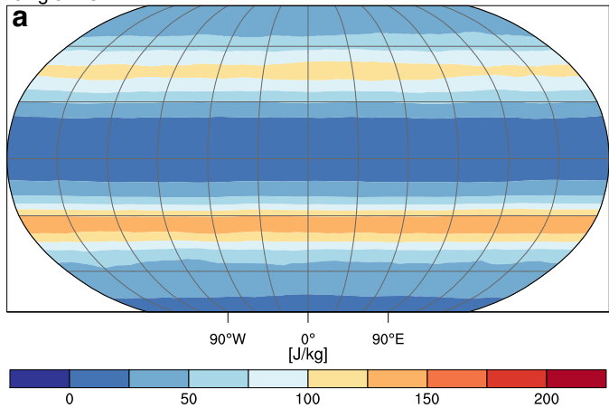
single ITCZ
