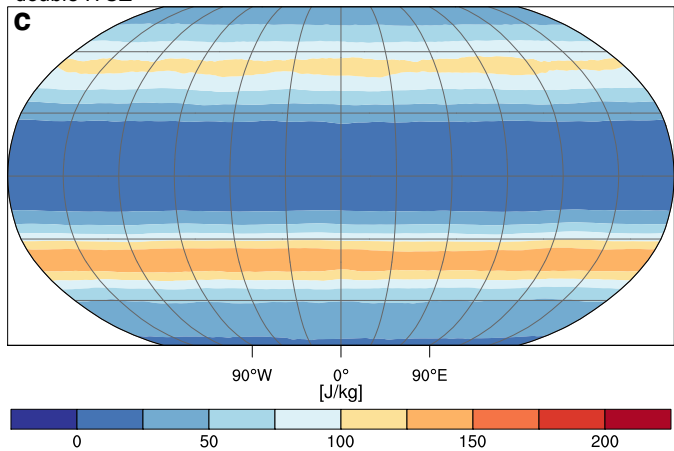
double ITCZ
