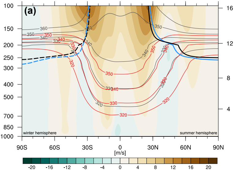
double ITCZ
