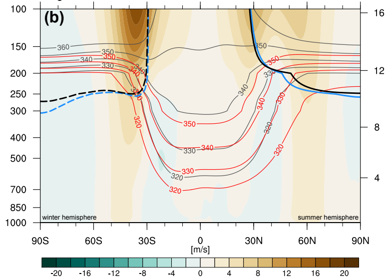
single ITCZ
