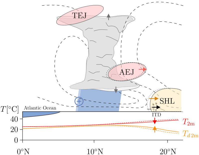
(c) c_soil
