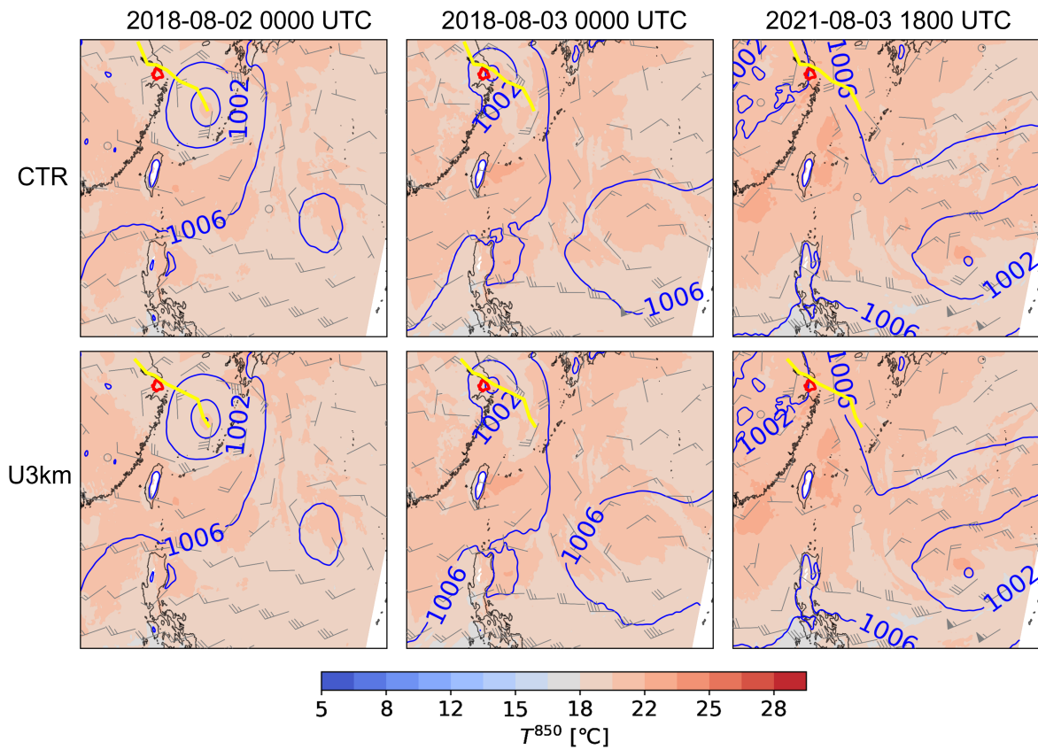
Figure S4. Same as Figure 9 in the manuscript but for typhoon Jongdari.
