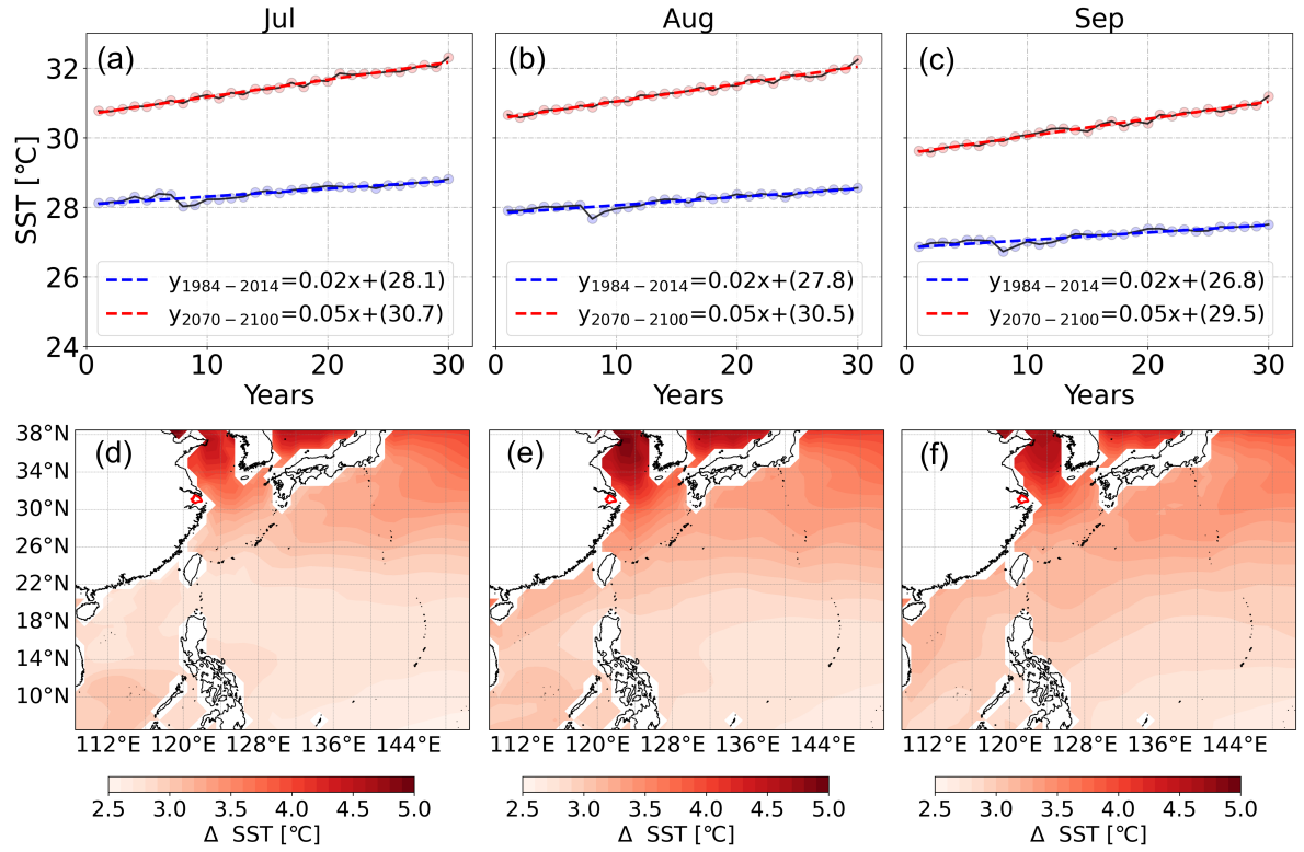
Figure S1. Comparing the average SST for the months of July (a)(d), August (b)(e), and September (c)(f) between the CMIP6 historical period (1984-2014) and the future period (2070-2100) under the SSP-8.5 high-emission. The first row represents the temporal trend of SST, while the second row shows the spatial difference of SST in domain DO1.
