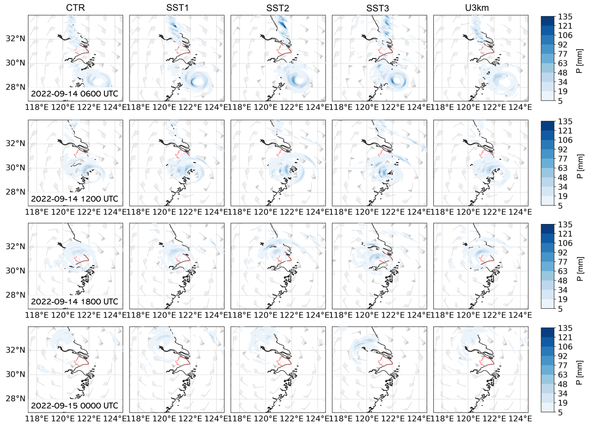
Figure S3. An example (Typhoon Muifa) of the WRF-simulated hourly rainfall ( P [mm]) and 850 hPa height wind velocity ( W^{850} [m s -1 ]) at several time steps under different scenarios. Shanghai area is marked in red.
