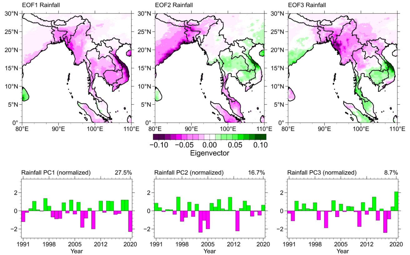
Fig S3 First three EOF modes of October rainfall and their normalized PCs over the study area, with a focus on rainfall variability in mainland Indochina. This figure was created with Python 3.10 (Matplotlib 3.5.2 https://matplotlib.org/ , Cartopy 0.20.0 https://pypi.org/project/Cartopy/ ).
