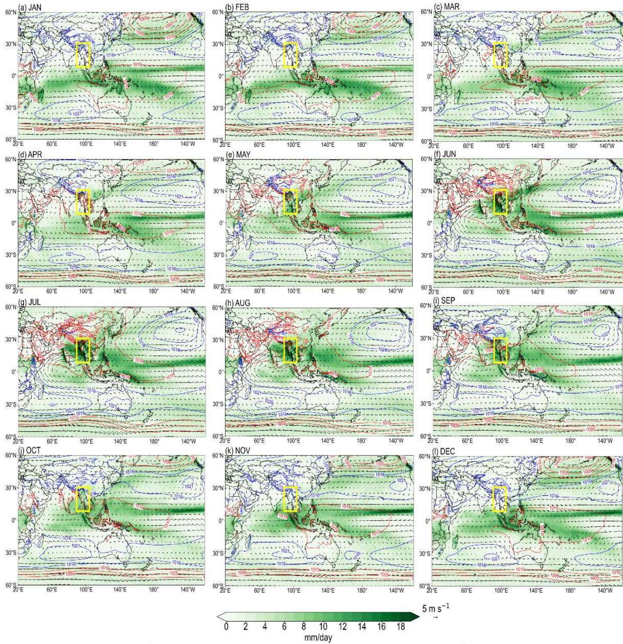
Fig S5 Climatology intraseasonal variation of rainfall (shade, mm), 850 hPa wind (vector, m/s) and geopotential (contour, gpm). This figure was created with Python 3.10 (Matplotlib 3.5.2 [ https://matplotlib.org/ ], Cartopy 0.20.0 [ https://pypi.org/project/Cartopy/ ]).
