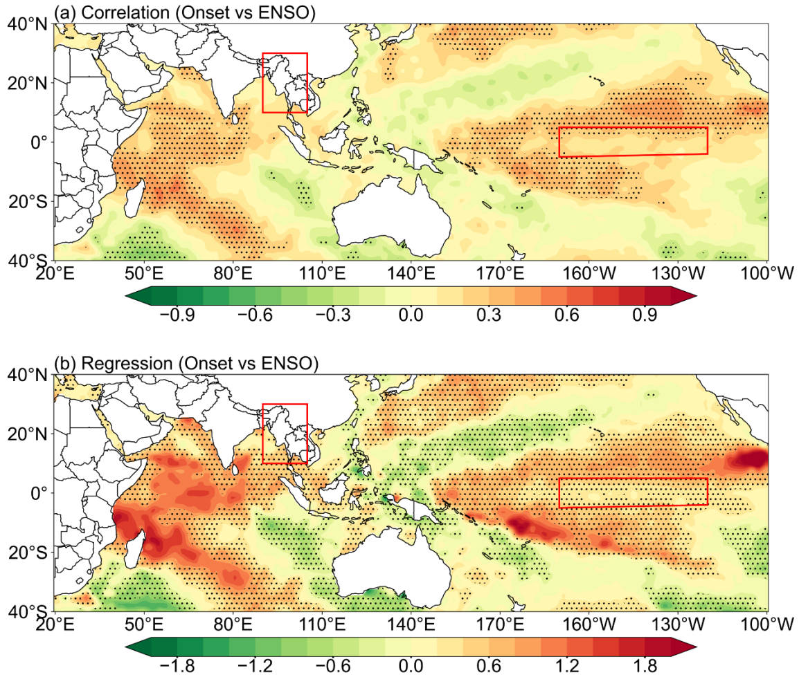
Fig S10 (a) Correlation between sea surface temperatures (SSTs) and MSWM onset dates, (b) similar as (a) but for regression. Dotted hatches mean 95% confident area by t-test statically. This figure was created with Python 3.10 (Matplotlib 3.5.2 [ https://matplotlib.org/ ], Cartopy 0.20.0 [ https://pypi.org/project/Cartopy/ ]).
