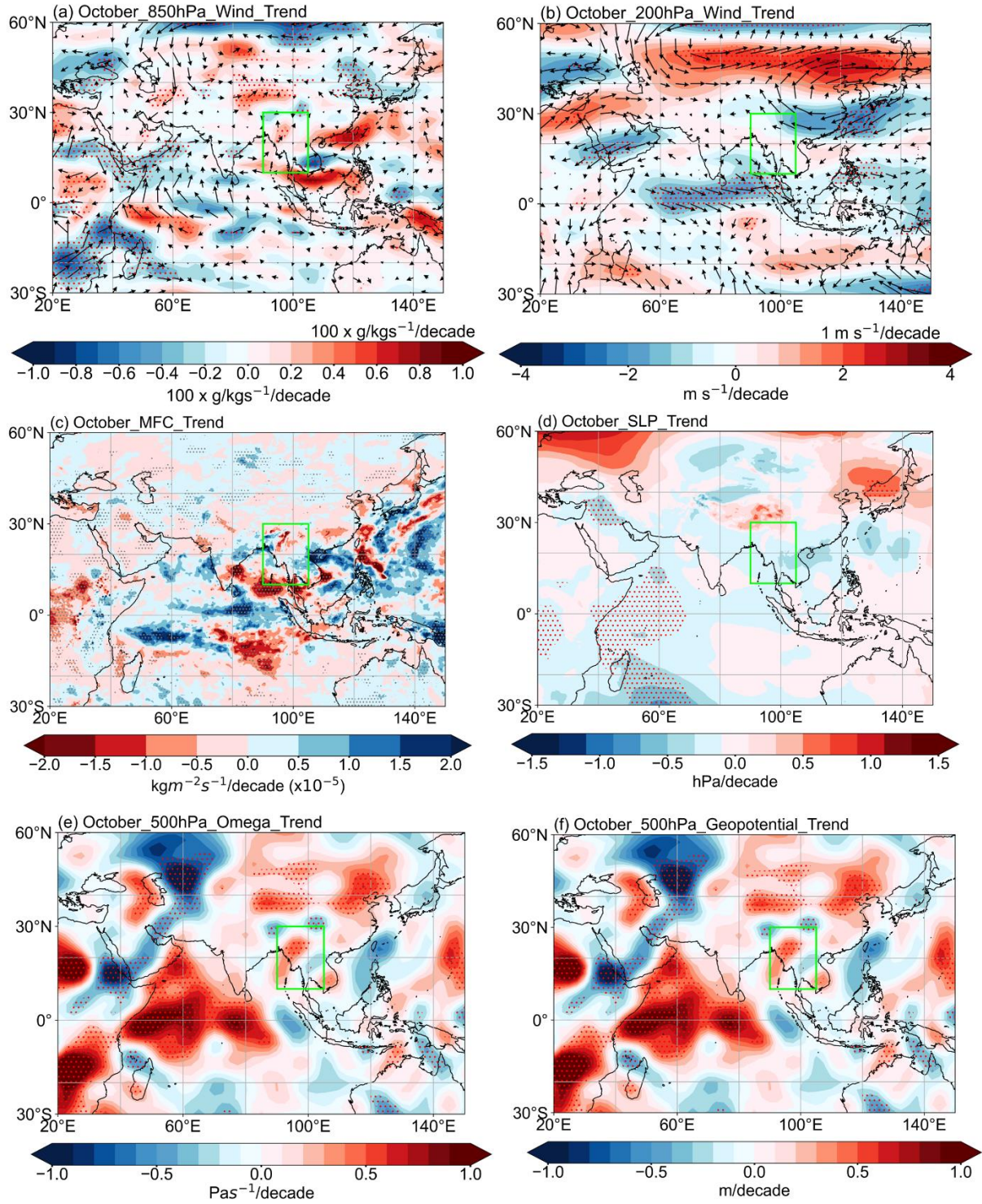
Fig S7 Spatial trend analysis of October (a) 850 hPa wind, (b) 200 hPa wind, (c) MFC, (d) SLP, (e) 500 hPa Omega, and (f) 500 hPa geopotential, illustrating evolving atmospheric dynamics over mainland Indochina. This figure was created with Python 3.10 (Matplotlib 3.5.2 [ https://matplotlib.org/ ], Cartopy 0.20.0 [ https://pypi.org/project/Cartopy/ ]).
