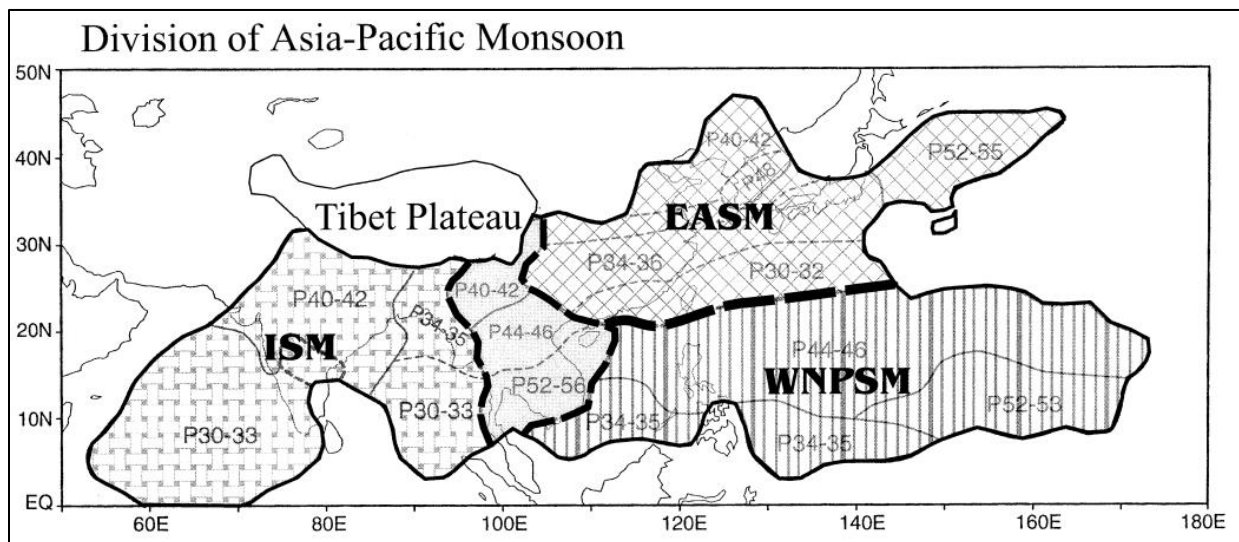
Fig S1 Three subregions make up the Asian-Pacific monsoon (B. Wang & Ho, 2002)
