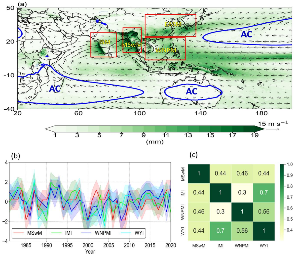
Fig S6 Four sub-regions of Asian-Pacific monsoon adopted from (Wang & Ho, 2002). ISM, MSwM, and WNPSM are tropical monsoon regions and the subtropical monsoon, EASM by shaded daily rainfall (mm/day) with 850 hPa level wind (m/s) and 15000-gpm geopotential contour blue line. (b) Annual time series of indices and (c) their correlation heatmap. This figure was created with Python 3.10 (Matplotlib 3.5.2 [ https://matplotlib.org/ ], Cartopy 0.20.0 [ https://pypi.org/project/Cartopy/ ]).
