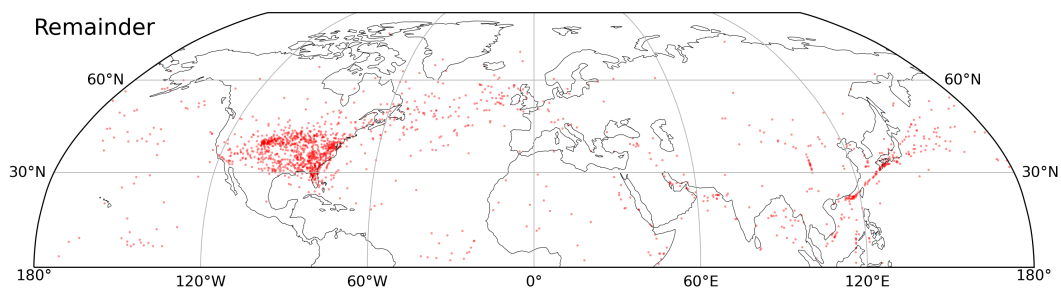
Figure S4. Geographical distribution of remainder events. The location of an event is determined by the report with the highest peak EDR value and each event is indicated by a red dot.
