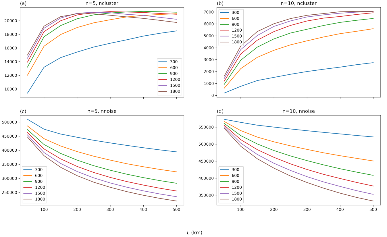
Figure S5. The number of clusters (ncluster) (a,b) and number of noise data points (nnoise) (c,d) identified by the DBSCAN algorithm as a function of L (km), with (a,c) N = 5 and (b,d) N = 10 . The values of T (in s) are indicated by the different colours of the curves.
